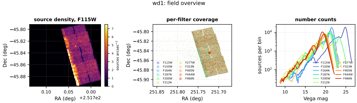
Figure 1: Overview of wd1. Left: source surface density in 72 \times 72 sky cells for F115W, the filter with the most detections. Centre: the sky coverage of each filter, sub-sampled. Right: number counts per filter; the peak of each curve is the turnover magnitude, the practical completeness limit beyond which the counts are set by detectability rather than by the stellar population.
