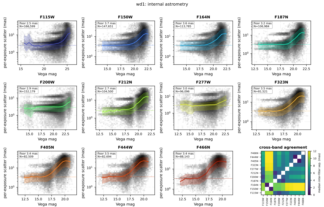
Figure 2: Internal astrometry of wd1. Per filter: the scatter of the individual-exposure centroids about the merged position, against brightness; greyscale is source density, the coloured line and band are the running median and 16–84th percentile, and the dotted line marks the bright-decile floor quoted in the panel. The final panel is the median separation between the same stars measured independently in each pair of filters; only sources independently detected in both bands are counted, since a forced or seeded position imported from another band would measure the merge radius rather than the astrometry.
