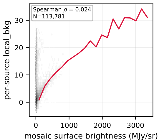
F200W: vs mosaic
