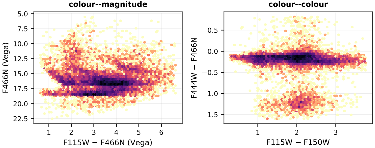
Figure 6: Colour diagrams for wd1, from the stage-m7 cross-band merge, in Vega magnitudes. These are differential between filters and so respond to systematics that per-filter statistics cannot see: a zero-point error shifts a sequence bodily, a saturation-correction discontinuity breaks it at a specific magnitude, and a filter-dependent background error tilts it.
