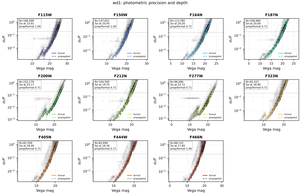
Figure 4: Photometric precision of wd1. Greyscale is source density; the solid line is the running median of the fitter’s formal uncertainty \sigma_F/F and the dashed line the same quantity propagated from the per-exposure scatter. The dotted horizontal line is \sigma_F/F = 0.2 , and where the median crosses it is quoted as the 5\sigma depth. A propagated-to-formal ratio above unity means the exposures disagree by more than the fit covariance predicts.
