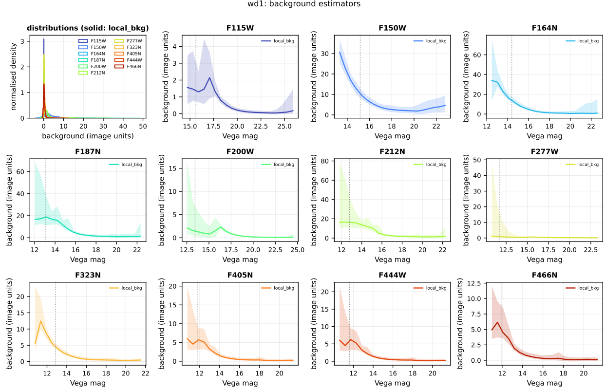
Figure 7: Background estimators for wd1. First panel: the distribution of the annulus background handed to the fitter (solid) and, where available, the residual-footprint background (dashed). Remaining panels: the running median of each against brightness, with the 16–84th percentile band for the annulus estimator; the vertical dotted line marks the brightest 1 per cent, where a star's own wings begin to enter its own background aperture. The residual-footprint column is present for 0 of 11 filters; it was added in 2026-07, so catalogues produced before then carry only the annulus estimator.
