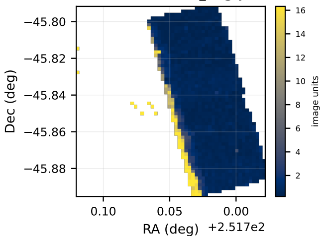
F200W: median local_bkg per cell
