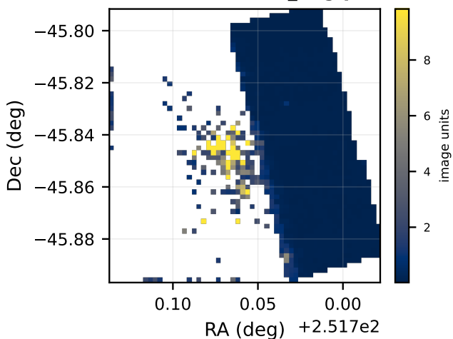
F164N: median local_bkg per cell
