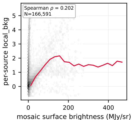
F164N: vs mosaic
