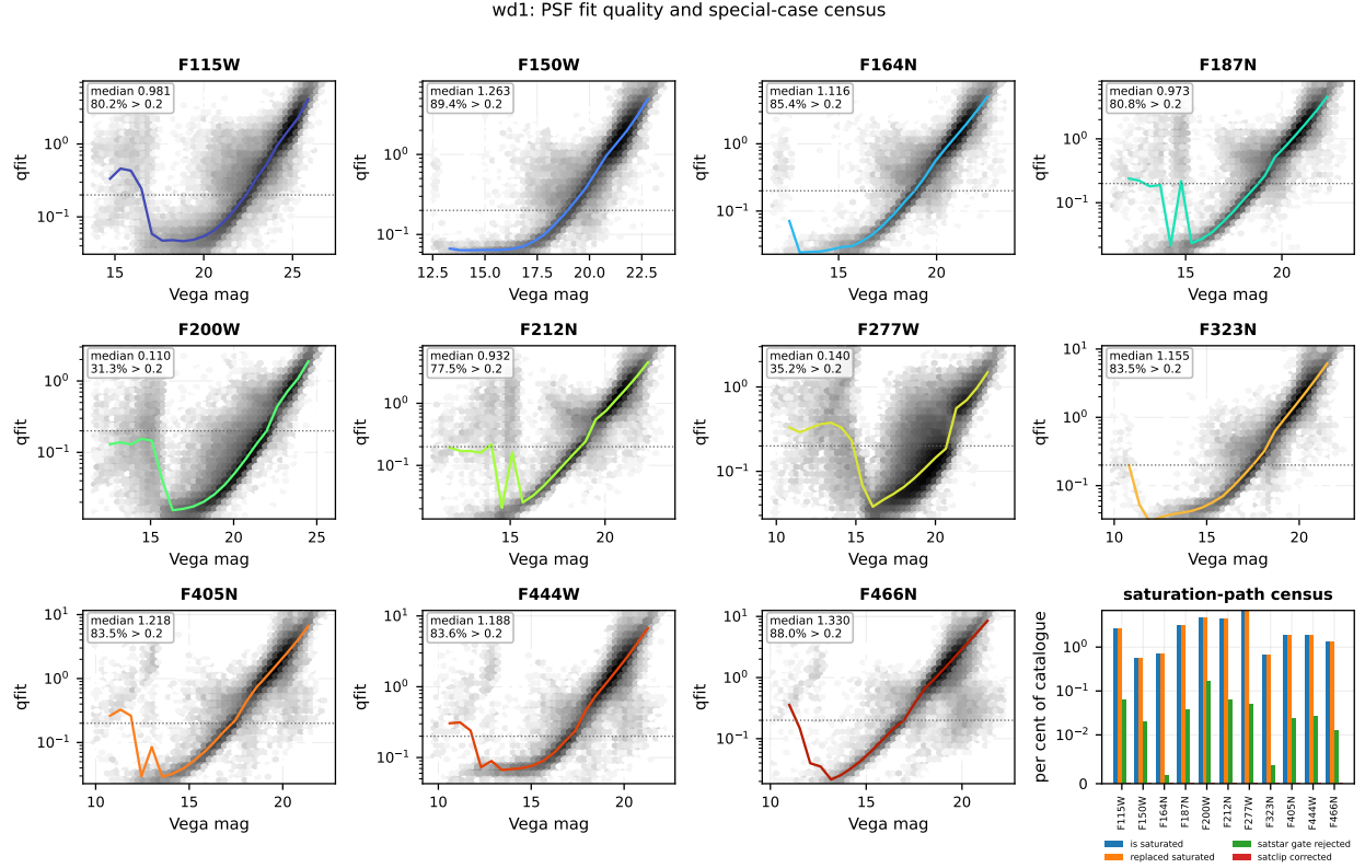
Figure 5: PSF-fit quality for wd1. Per filter, the normalised fit residual qfit against brightness (greyscale: source density; line: running median; dotted: the qfit = 0.2 vetting threshold). The final panel is the fraction of each filter’s catalogue touched by the saturation-handling paths: flagged saturated, core-replaced, rejected by the saturated-star gate, and clip-corrected.
