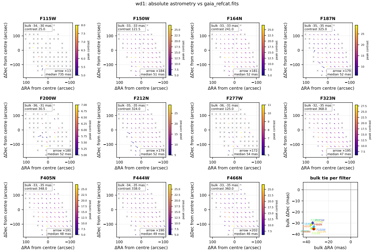
Figure 3: Absolute astrometry of wd1 against its registered reference catalogue. Each per-filter panel maps the offset-histogram tie on a 12×12 tile grid (arrows, exaggerated; colour is the per-tile peak contrast), with the whole-field bulk tie quoted in the corner. Grey crosses mark tiles whose tie was only found by widening the search window and whose offset is therefore not trustworthy. The final panel collects the bulk ties. Offsets are measured by offset-histogram stacking, which is immune to the nearest-neighbour pairing collapse that a median against a dense reference suffers; the per-tile map is shown because a bulk offset near zero does not by itself mean the field is registered.
