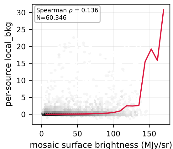
F360M: vs mosaic
