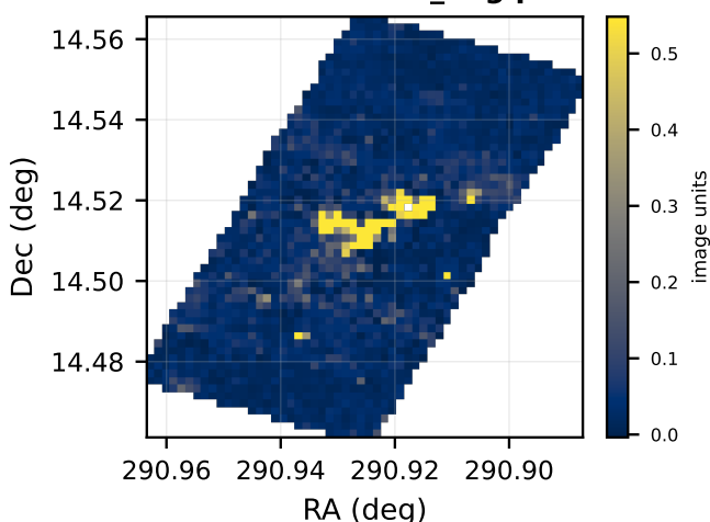
F405N: median local_bkg per cell
