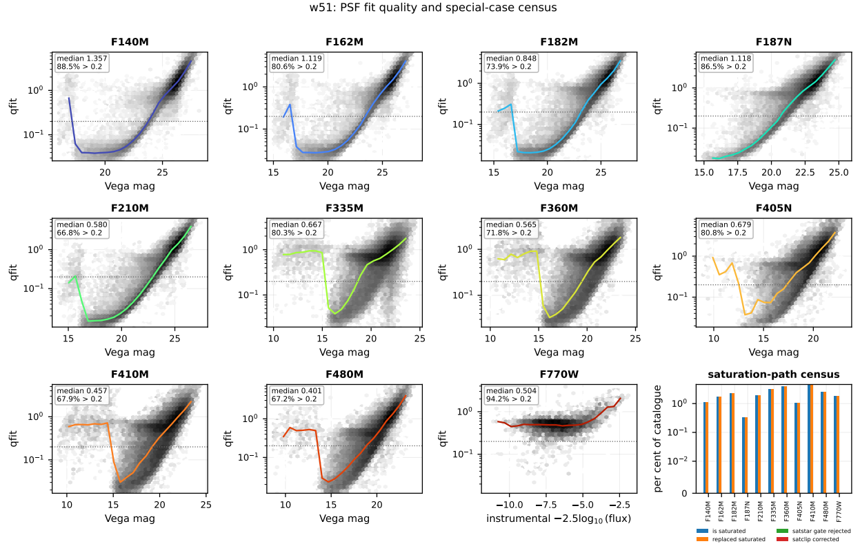
Figure 5: PSF-fit quality for w51. Per filter, the normalised fit residual qfit against brightness (greyscale: source density; line: running median; dotted: the qfit = 0.2 vetting threshold). The final panel is the fraction of each filter’s catalogue touched by the saturation-handling paths: flagged saturated, core-replaced, rejected by the saturated-star gate, and clip-corrected.
