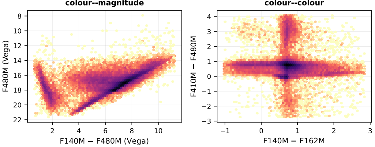
Figure 6: Colour diagrams for w51, from the stage-m8 cross-band merge, in Vega magnitudes. These are differential between filters and so respond to systematics that per-filter statistics cannot see: a zero-point error shifts a sequence bodily, a saturation-correction discontinuity breaks it at a specific magnitude, and a filter-dependent background error tilts it.
