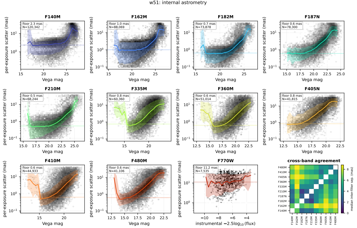
Figure 2: Internal astrometry of w51. Per filter: the scatter of the individual-exposure centroids about the merged position, against brightness; greyscale is source density, the coloured line and band are the running median and 16–84th percentile, and the dotted line marks the bright-decile floor quoted in the panel. The final panel is the median separation between the same stars measured independently in each pair of filters; only sources independently detected in both bands are counted, since a forced or seeded position imported from another band would measure the merge radius rather than the astrometry.
