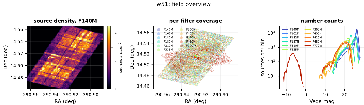
Figure 1: Overview of w51. Left: source surface density in 72 \times 72 sky cells for F140M, the filter with the most detections. Centre: the sky coverage of each filter, sub-sampled. Right: number counts per filter; the peak of each curve is the turnover magnitude, the practical completeness limit beyond which the counts are set by detectability rather than by the stellar population.
