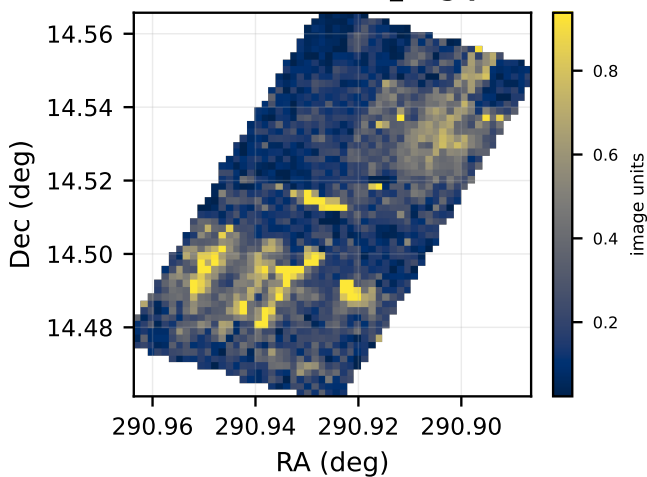
F335M: median local_bkg per cell
