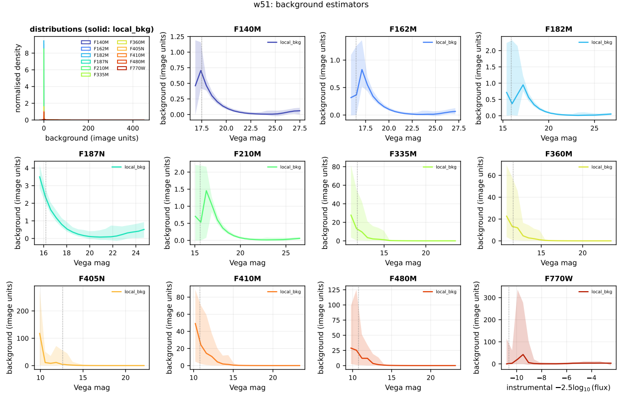
Figure 7: Background estimators for w51. First panel: the distribution of the annulus background handed to the fitter (solid) and, where available, the residual-footprint background (dashed). Remaining panels: the running median of each against brightness, with the 16–84th percentile band for the annulus estimator; the vertical dotted line marks the brightest 1 per cent, where a star's own wings begin to enter its own background aperture. The residual-footprint column is present for 0 of 11 filters; it was added in 2026-07, so catalogues produced before then carry only the annulus estimator.
