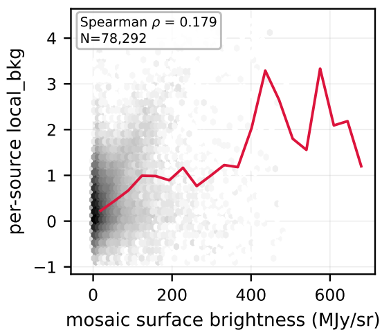
F335M: vs mosaic
