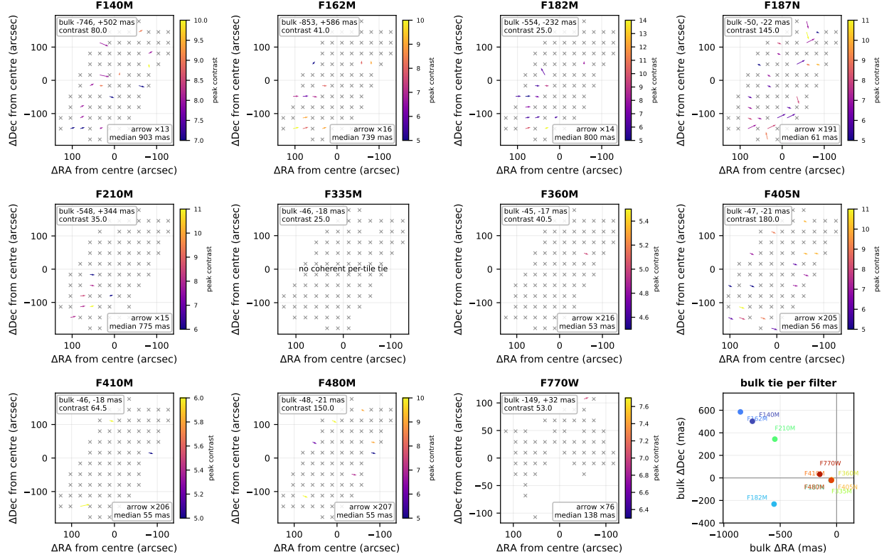
Figure 3: Absolute astrometry of w51 against its registered reference catalogue. Each per-filter panel maps the offset-histogram tie on a 12 \times 12 tile grid (arrows, exaggerated; colour is the per-tile peak contrast), with the whole-field bulk tie quoted in the corner. Grey crosses mark tiles whose tie was only found by widening the search window and whose offset is therefore not trustworthy. The final panel collects the bulk ties. Offsets are measured by offset-histogram stacking, which is immune to the nearest-neighbour pairing collapse that a median against a dense reference suffers; the per-tile map is shown because a bulk offset near zero does not by itself mean the field is registered.
