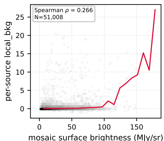
F405N: vs mosaic
