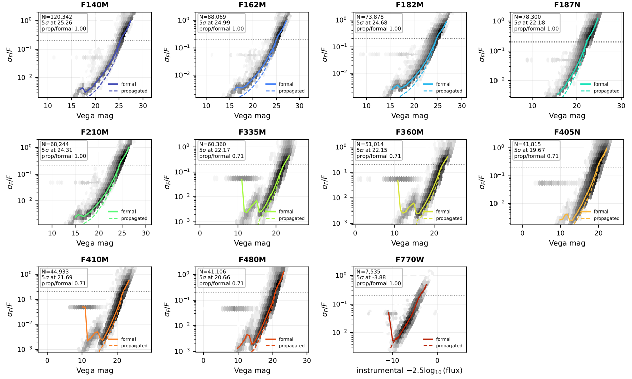
Figure 4: Photometric precision of w51. Greyscale is source density; the solid line is the running median of the fitter’s formal uncertainty \sigma_F/F and the dashed line the same quantity propagated from the per-exposure scatter. The dotted horizontal line is \sigma_F/F = 0.2 , and where the median crosses it is quoted as the 5\sigma depth. A propagated-to-formal ratio above unity means the exposures disagree by more than the fit covariance predicts.
