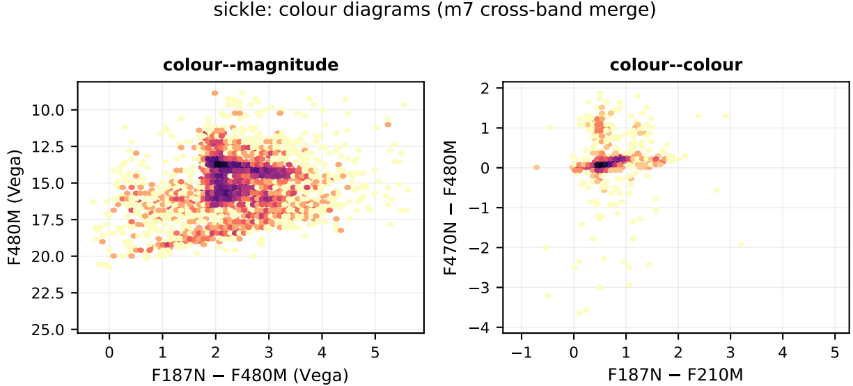
Figure 6: Colour diagrams for sickle, from the stage-m7 cross-band merge, in Vega magnitudes. These are differential between filters and so respond to systematics that per-filter statistics cannot see: a zero-point error shifts a sequence bodily, a saturation-correction discontinuity breaks it at a specific magnitude, and a filter-dependent background error tilts it.
