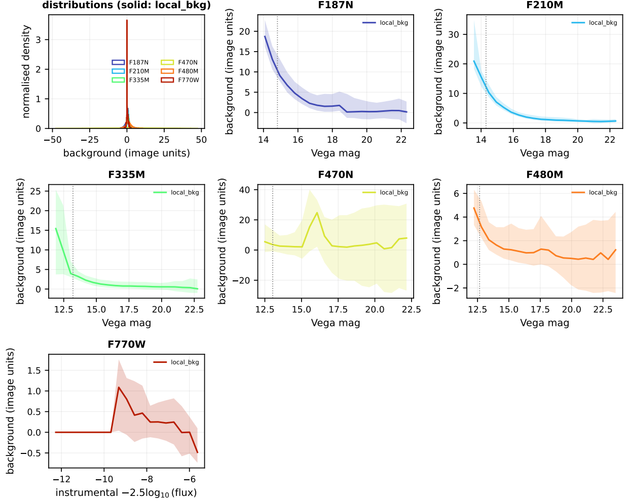
Figure 7: Background estimators for sickle. First panel: the distribution of the annulus background handed to the fitter (solid) and, where available, the residual-footprint background (dashed). Remaining panels: the running median of each against brightness, with the 16–84th percentile band for the annulus estimator; the vertical dotted line marks the brightest 1 per cent, where a star’s own wings begin to enter its own background aperture. The residual-footprint column is present for 0 of 6 filters; it was added in 2026-07, so catalogues produced before then carry only the annulus estimator.
