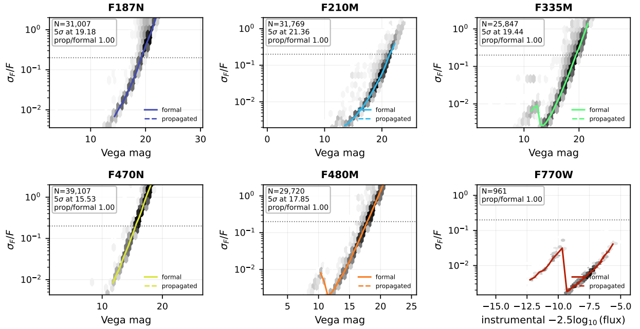
Figure 4: Photometric precision of sickle. Greyscale is source density; the solid line is the running median of the fitter’s formal uncertainty \sigma_F/F and the dashed line the same quantity propagated from the per-exposure scatter. The dotted horizontal line is \sigma_F/F = 0.2 , and where the median crosses it is quoted as the 5 \sigma depth. A propagated-to-formal ratio above unity means the exposures disagree by more than the fit covariance predicts.
