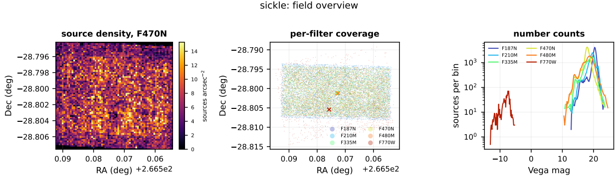
Figure 1: Overview of sickle. Left: source surface density in 72 \times 72 sky cells for F470N, the filter with the most detections. Centre: the sky coverage of each filter, sub-sampled. Right: number counts per filter; the peak of each curve is the turnover magnitude, the practical completeness limit beyond which the counts are set by detectability rather than by the stellar population.
