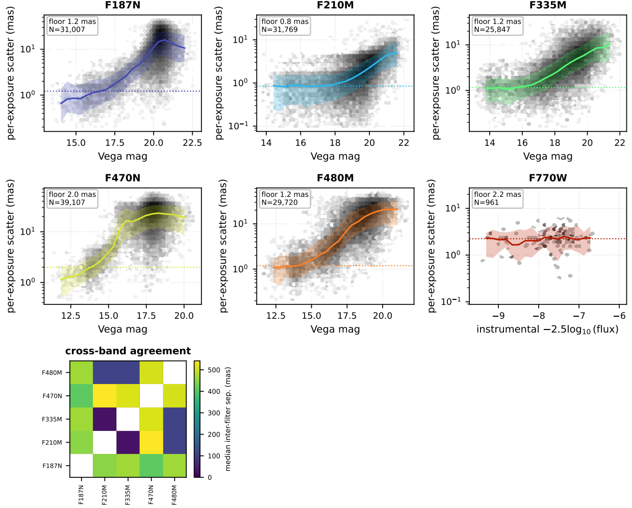
Figure 2: Internal astrometry of sickle. Per filter: the scatter of the individual-exposure centroids about the merged position, against brightness; greyscale is source density, the coloured line and band are the running median and 16–84th percentile, and the dotted line marks the bright-decade floor quoted in the panel. The final panel is the median separation between the same stars measured independently in each pair of filters; only sources independently detected in both bands are counted, since a forced or seeded position imported from another band would measure the merge radius rather than the astrometry.
