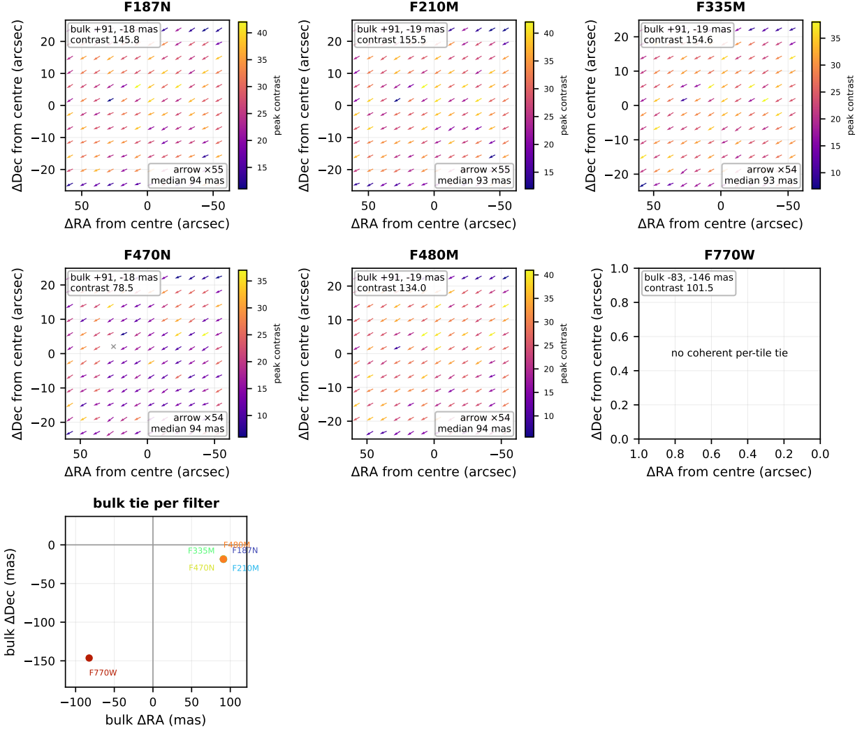
Figure 3: Absolute astrometry of sickle against its registered reference catalogue. Each per-filter panel maps the offset-histogram tie on a 12 \times 12 tile grid (arrows, exaggerated; colour is the per-tile peak contrast), with the whole-field bulk tie quoted in the corner. Grey crosses mark tiles whose tie was only found by widening the search window and whose offset is therefore not trustworthy. The final panel collects the bulk ties. Offsets are measured by offset-histogram stacking, which is immune to the nearest-neighbour pairing collapse that a median against a dense reference suffers; the per-tile map is shown because a bulk offset near zero does not by itself mean the field is registered.
