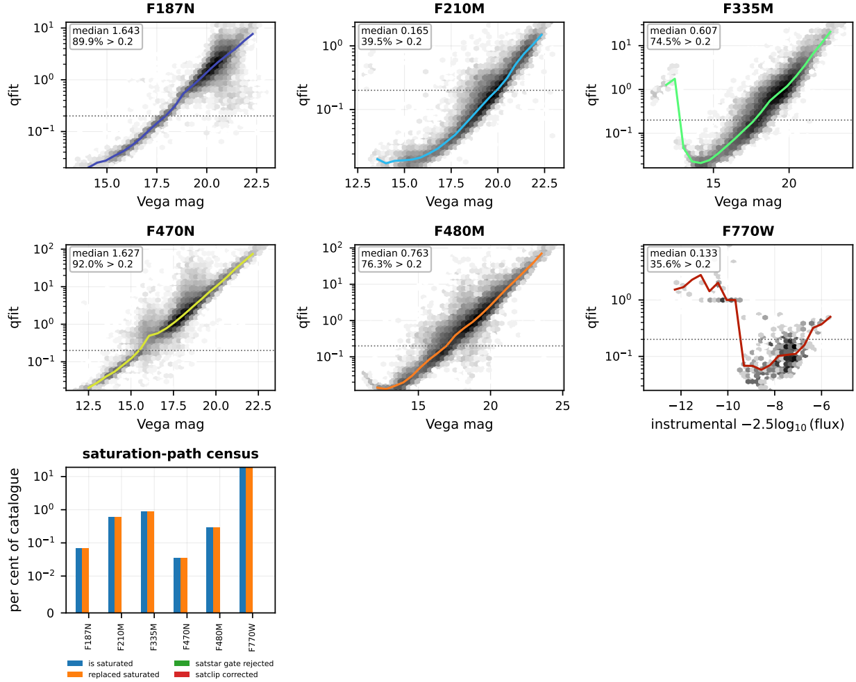
Figure 5: PSF-fit quality for sickle. Per filter, the normalised fit residual q_{\text{fit}} against brightness (greyscale: source density; line: running median; dotted: the q_{\text{fit}} = 0.2 vetting threshold). The final panel is the fraction of each filter's catalogue touched by the saturation-handling paths: flagged saturated, core-replaced, rejected by the saturated-star gate, and clip-corrected.
