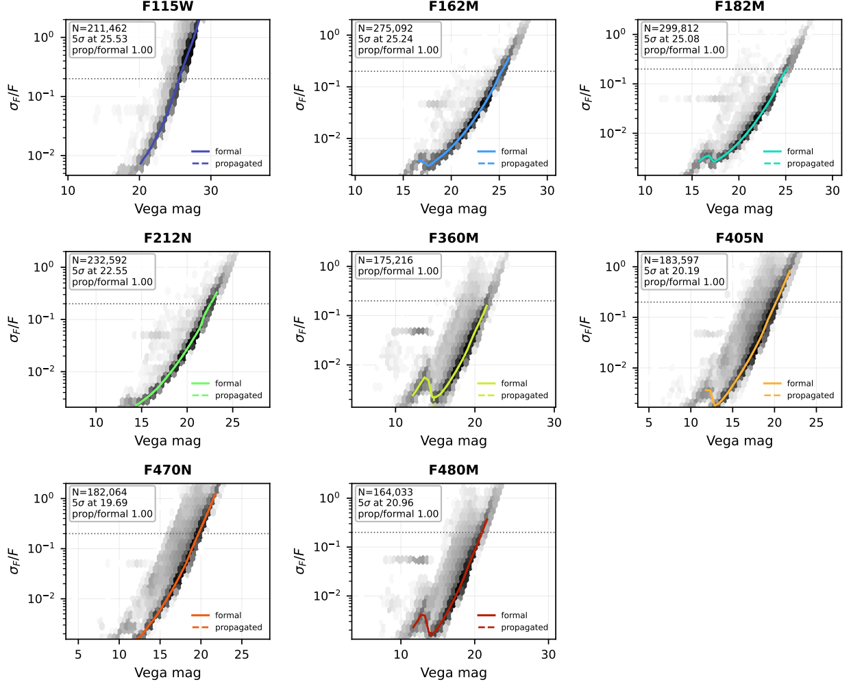
Figure 4: Photometric precision of sgrc. Greyscale is source density; the solid line is the running median of the fitter’s formal uncertainty \sigma_F/F and the dashed line the same quantity propagated from the per-exposure scatter. The dotted horizontal line is \sigma_F/F = 0.2 , and where the median crosses it is quoted as the 5 \sigma depth. A propagated-to-formal ratio above unity means the exposures disagree by more than the fit covariance predicts.
