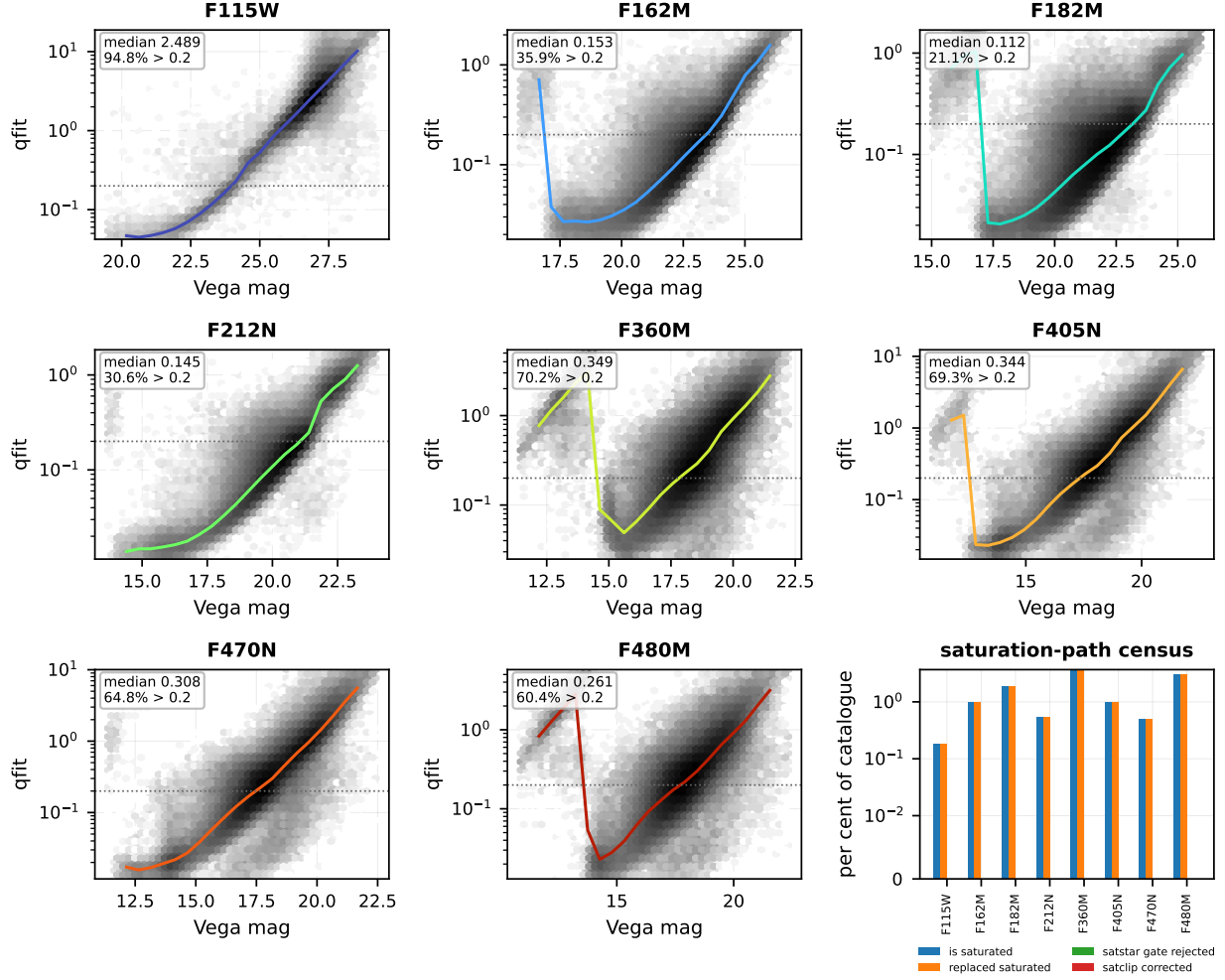
Figure 5: PSF-fit quality for sgrc. Per filter, the normalised fit residual q_{\text{fit}} against brightness (greyscale: source density; line: running median; dotted: the q_{\text{fit}} = 0.2 vetting threshold). The final panel is the fraction of each filter's catalogue touched by the saturation-handling paths: flagged saturated, core-replaced, rejected by the saturated-star gate, and clip-corrected.
