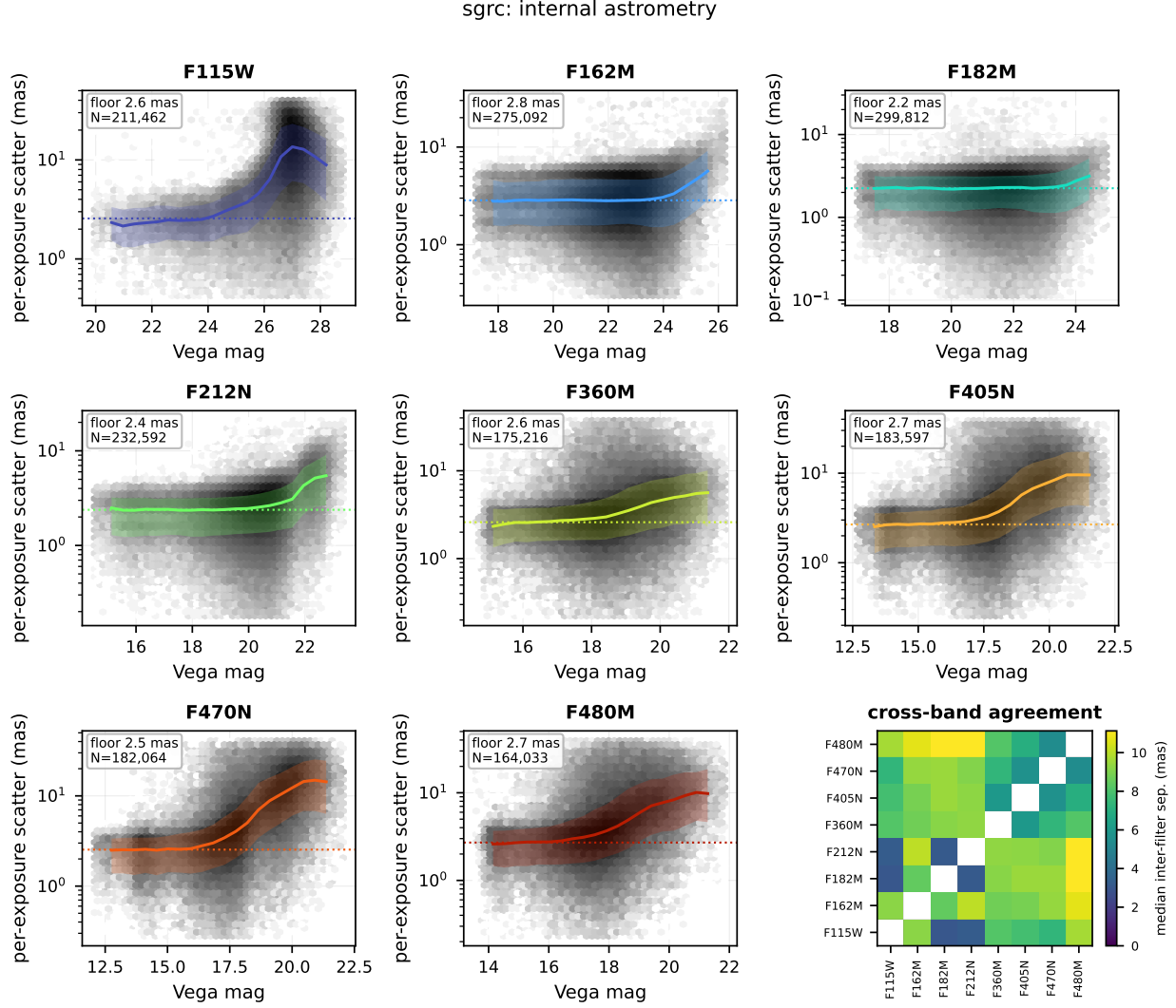
Figure 2: Internal astrometry of sgrc. Per filter: the scatter of the individual-exposure centroids about the merged position, against brightness; greyscale is source density, the coloured line and band are the running median and 16–84th percentile, and the dotted line marks the bright-decade floor quoted in the panel. The final panel is the median separation between the same stars measured independently in each pair of filters; only sources independently detected in both bands are counted, since a forced or seeded position imported from another band would measure the merge radius rather than the astrometry.
