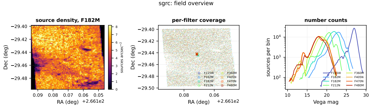
Figure 1: Overview of sgrc. Left: source surface density in 72 \times 72 sky cells for F182M, the filter with the most detections. Centre: the sky coverage of each filter, sub-sampled. Right: number counts per filter; the peak of each curve is the turnover magnitude, the practical completeness limit beyond which the counts are set by detectability rather than by the stellar population.
