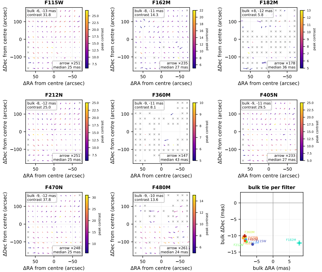
Figure 3: Absolute astrometry of sgrc against its registered reference catalogue. Each per-filter panel maps the offset-histogram tie on a 12×12 tile grid (arrows, exaggerated; colour is the per-tile peak contrast), with the whole-field bulk tie quoted in the corner. Grey crosses mark tiles whose tie was only found by widening the search window and whose offset is therefore not trustworthy. The final panel collects the bulk ties. Offsets are measured by offset-histogram stacking, which is immune to the nearest-neighbour pairing collapse that a median against a dense reference suffers; the per-tile map is shown because a bulk offset near zero does not by itself mean the field is registered.
