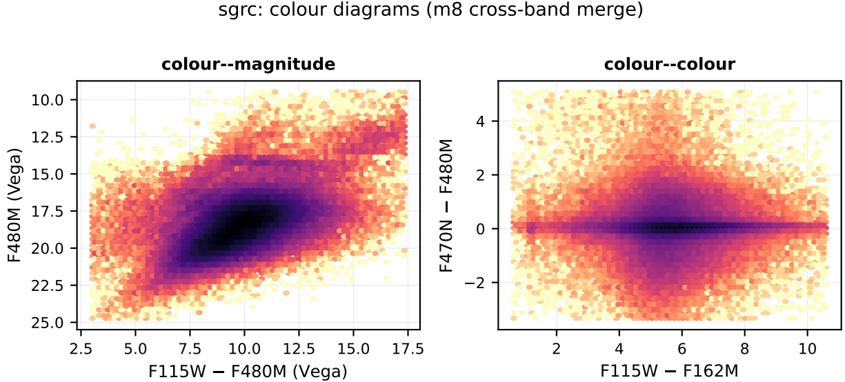
Figure 6: Colour diagrams for sgrc, from the stage-m8 cross-band merge, in Vega magnitudes. These are differential between filters and so respond to systematics that per-filter statistics cannot see: a zero-point error shifts a sequence bodily, a saturation-correction discontinuity breaks it at a specific magnitude, and a filter-dependent background error tilts it.
