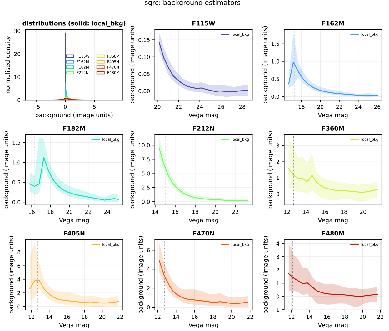
Figure 7: Background estimators for sgrc . First panel: the distribution of the annulus background handed to the fitter (solid) and, where available, the residual-footprint background (dashed). Remaining panels: the running median of each against brightness, with the 16–84th percentile band for the annulus estimator; the vertical dotted line marks the brightest 1 per cent, where a star’s own wings begin to enter its own background aperture. The residual-footprint column is present for 0 of 8 filters; it was added in 2026-07, so catalogues produced before then carry only the annulus estimator.
