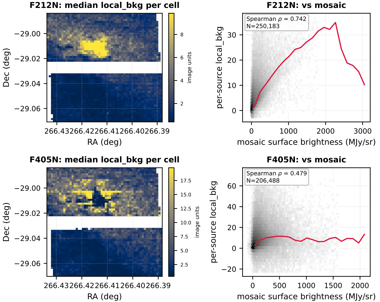
Figure 8: Spatial background structure in sgra. Left column: the median per-source background in 56 \times 56 sky cells – a map of the diffuse emission built entirely from the star catalogue. Right column: the same per-source value against the surface brightness of the drizzled mosaic sampled at that source’s position, with the running median in red and the Spearman rank correlation quoted. A high rank correlation is the evidence that the per-source background is measuring the astrophysical extended emission rather than a fitting artefact.
