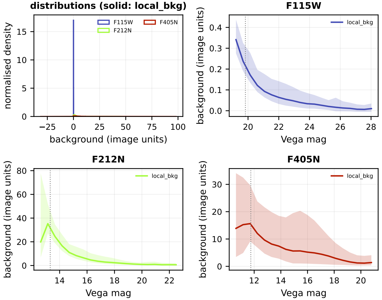
Figure 7: Background estimators for sgra. First panel: the distribution of the annulus background handed to the fitter (solid) and, where available, the residual-footprint background (dashed). Remaining panels: the running median of each against brightness, with the 16–84th percentile band for the annulus estimator; the vertical dotted line marks the brightest 1 per cent, where a star’s own wings begin to enter its own background aperture. The residual-footprint column is present for 0 of 3 filters; it was added in 2026-07, so catalogues produced before then carry only the annulus estimator.
