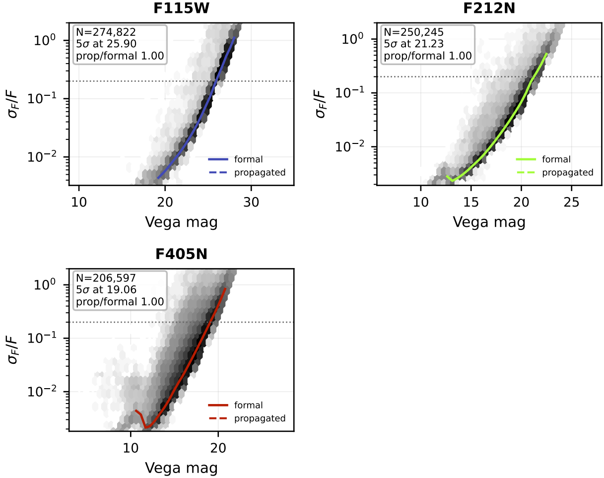
Figure 4: Photometric precision of sgra. Greyscale is source density; the solid line is the running median of the fitter’s formal uncertainty \sigma_F/F and the dashed line the same quantity propagated from the per-exposure scatter. The dotted horizontal line is \sigma_F/F = 0.2 , and where the median crosses it is quoted as the 5\sigma depth. A propagated-to-formal ratio above unity means the exposures disagree by more than the fit covariance predicts.
