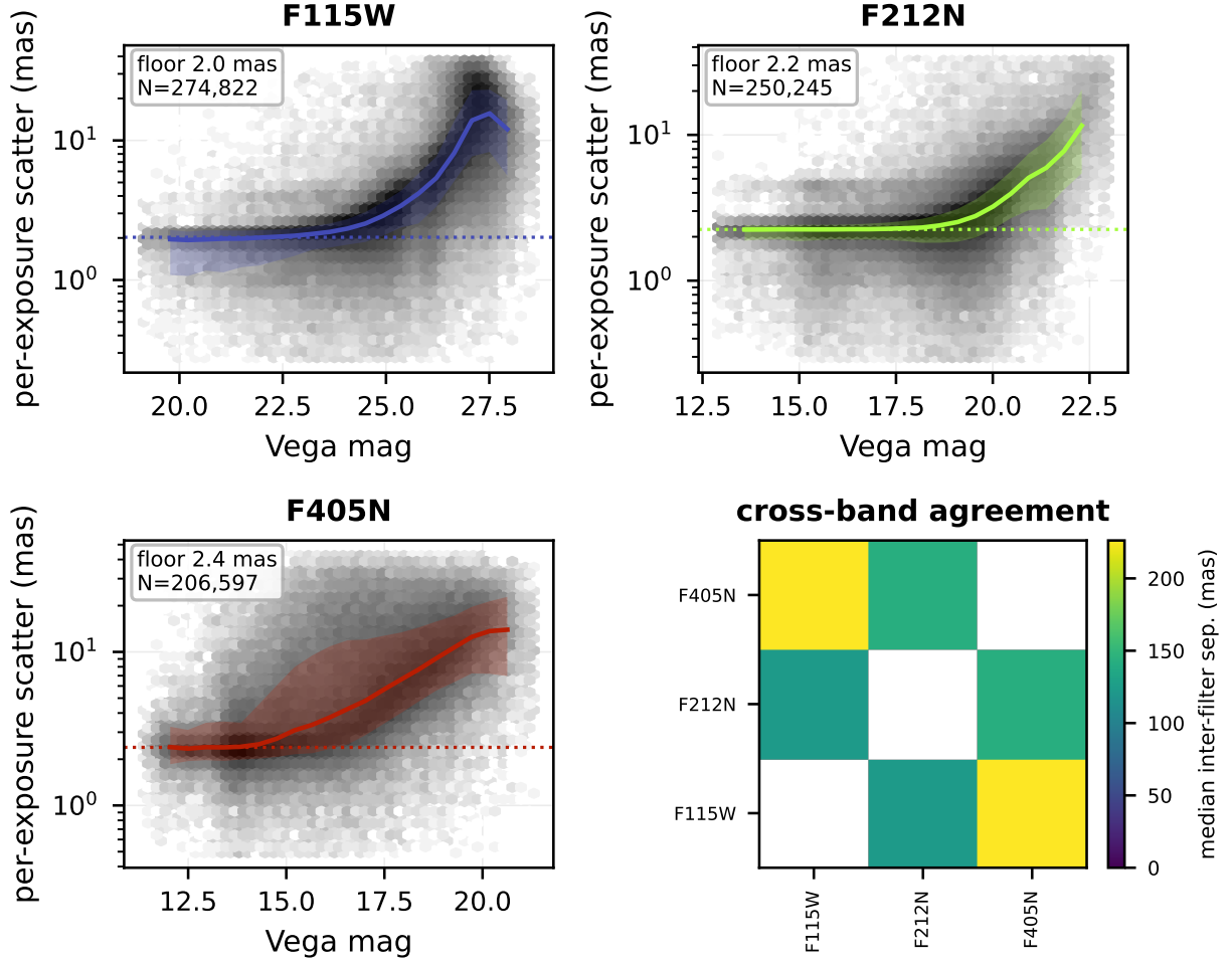
Figure 2: Internal astrometry of sgra. Per filter: the scatter of the individual-exposure centroids about the merged position, against brightness; greyscale is source density, the coloured line and band are the running median and 16–84th percentile, and the dotted line marks the bright-decade floor quoted in the panel. The final panel is the median separation between the same stars measured independently in each pair of filters; only sources independently detected in both bands are counted, since a forced or seeded position imported from another band would measure the merge radius rather than the astrometry.
