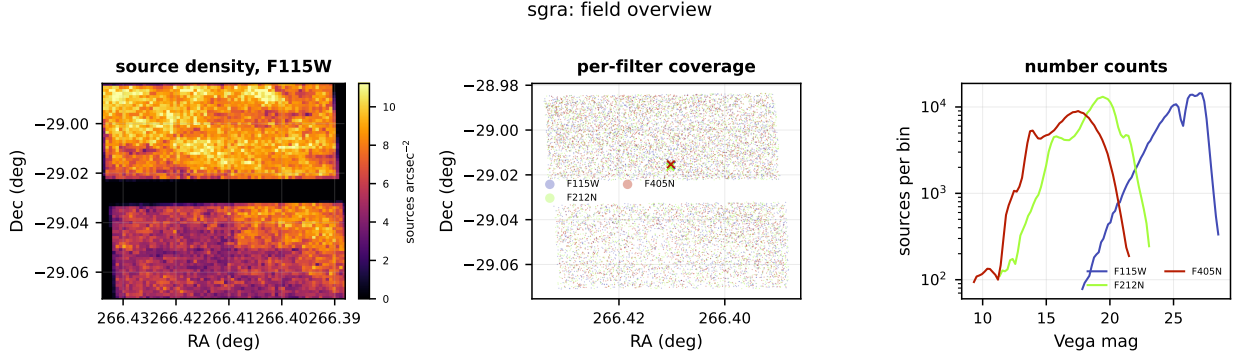
Figure 1: Overview of sgra. Left: source surface density in 72 \times 72 sky cells for F115W, the filter with the most detections. Centre: the sky coverage of each filter, sub-sampled. Right: number counts per filter; the peak of each curve is the turnover magnitude, the practical completeness limit beyond which the counts are set by detectability rather than by the stellar population.
