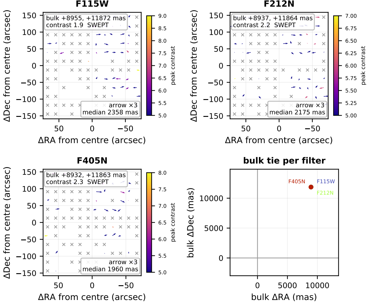
Figure 3: Absolute astrometry of sgra against its registered reference catalogue. Each per-filter panel maps the offset-histogram tie on a 12 \times 12 tile grid (arrows, exaggerated; colour is the per-tile peak contrast), with the whole-field bulk tie quoted in the corner. Grey crosses mark tiles whose tie was only found by widening the search window and whose offset is therefore not trustworthy. The final panel collects the bulk ties. Offsets are measured by offset-histogram stacking, which is immune to the nearest-neighbour pairing collapse that a median against a dense reference suffers; the per-tile map is shown because a bulk offset near zero does not by itself mean the field is registered.
