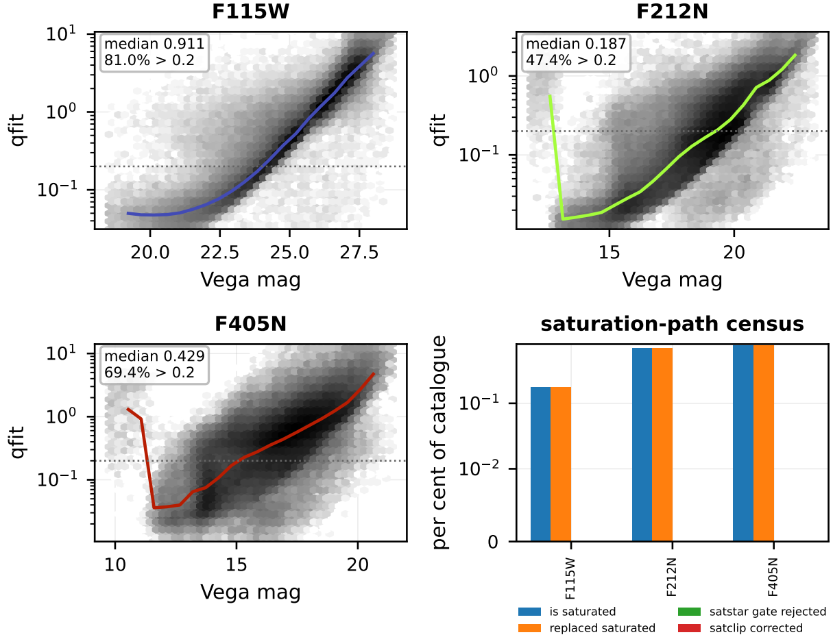
Figure 5: PSF-fit quality for sgra. Per filter, the normalised fit residual q_{\text{fit}} against brightness (greyscale: source density; line: running median; dotted: the q_{\text{fit}} = 0.2 vetting threshold). The final panel is the fraction of each filter's catalogue touched by the saturation-handling paths: flagged saturated, core-replaced, rejected by the saturated-star gate, and clip-corrected.
