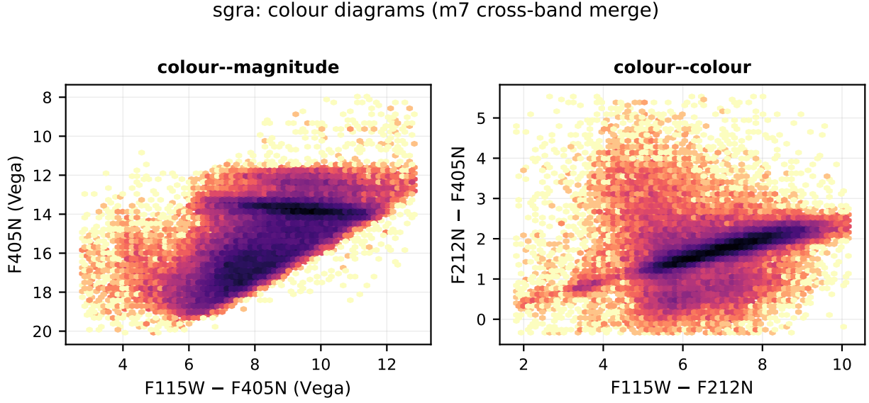
Figure 6: Colour diagrams for sgra, from the stage-m7 cross-band merge, in Vega magnitudes. These are differential between filters and so respond to systematics that per-filter statistics cannot see: a zero-point error shifts a sequence bodily, a saturation-correction discontinuity breaks it at a specific magnitude, and a filter-dependent background error tilts it.
