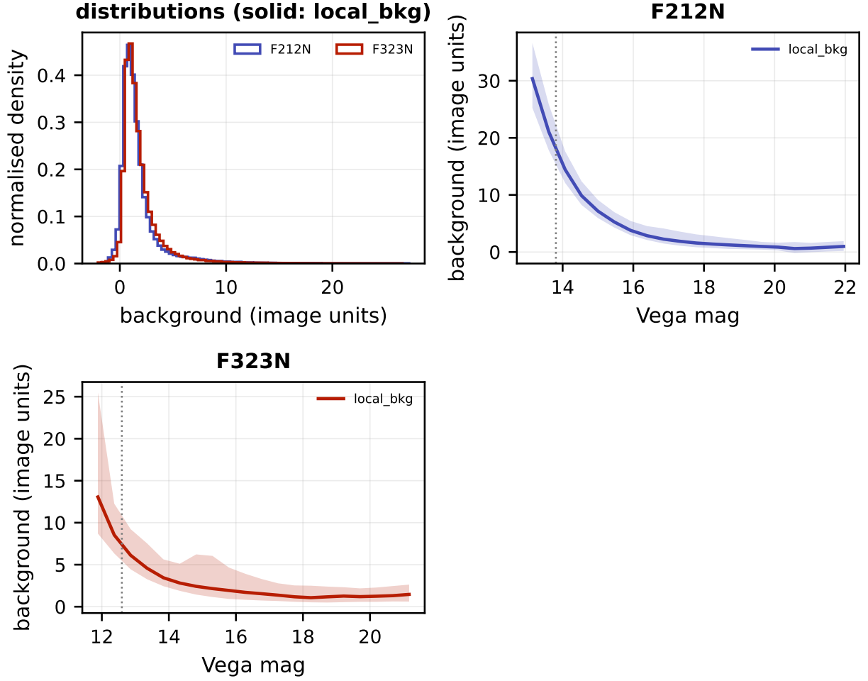
Figure 7: Background estimators for quintuplet. First panel: the distribution of the annulus background handed to the fitter (solid) and, where available, the residual-footprint background (dashed). Remaining panels: the running median of each against brightness, with the 16–84th percentile band for the annulus estimator; the vertical dotted line marks the brightest 1 per cent, where a star’s own wings begin to enter its own background aperture. The residual-footprint column is present for 0 of 2 filters; it was added in 2026-07, so catalogues produced before then carry only the annulus estimator.
