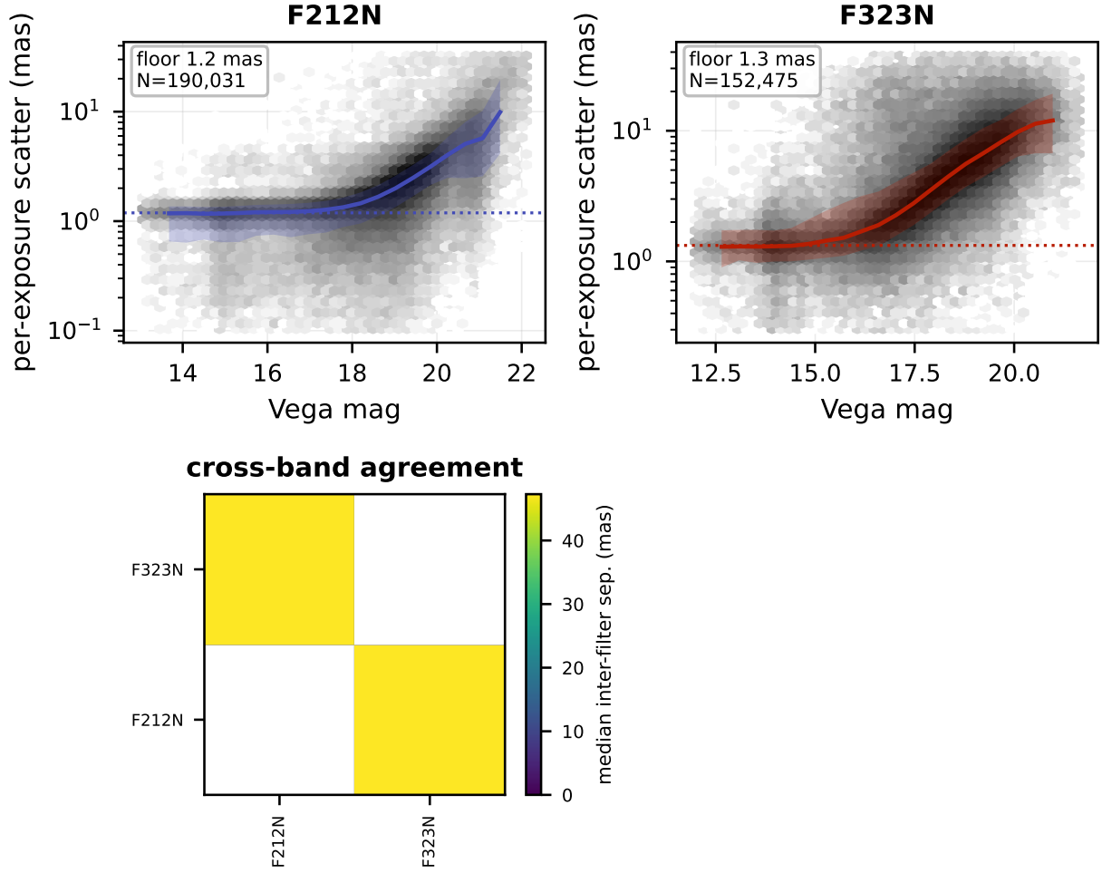
Figure 2: Internal astrometry of quintuplet. Per filter: the scatter of the individual-exposure centroids about the merged position, against brightness; greyscale is source density, the coloured line and band are the running median and 16–84th percentile, and the dotted line marks the bright-decile floor quoted in the panel. The final panel is the median separation between the same stars measured independently in each pair of filters; only sources independently detected in both bands are counted, since a forced or seeded position imported from another band would measure the merge radius rather than the astrometry.
