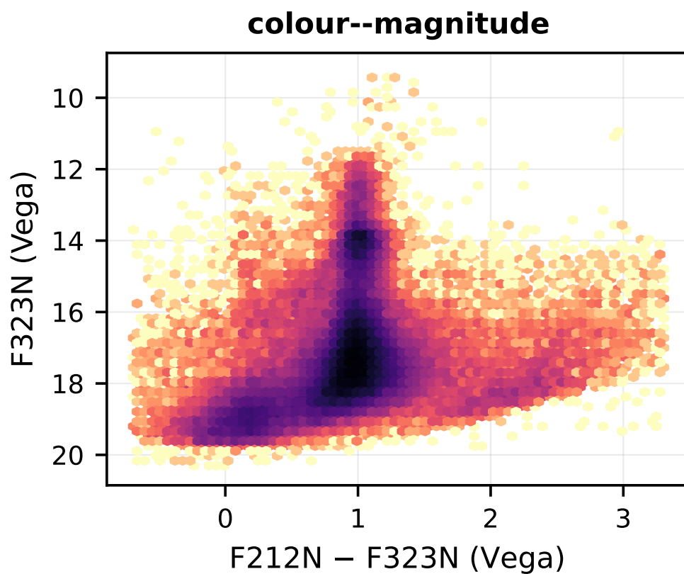
Figure 6: Colour diagrams for quintuplet, from the stage-m7 cross-band merge, in Vega magnitudes. These are differential between filters and so respond to systematics that per-filter statistics cannot see: a zero-point error shifts a sequence bodily, a saturation-correction discontinuity breaks it at a specific magnitude, and a filter-dependent background error tilts it.
