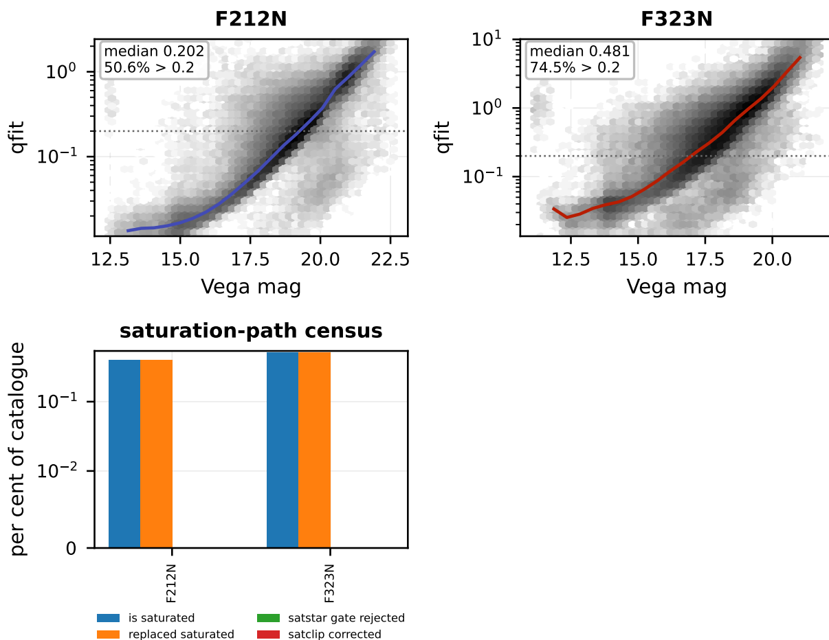
Figure 5: PSF-fit quality for quintuplet. Per filter, the normalised fit residual qfit against brightness (greyscale: source density; line: running median; dotted: the qfit = 0.2 vetting threshold). The final panel is the fraction of each filter's catalogue touched by the saturation-handling paths: flagged saturated, core-replaced, rejected by the saturated-star gate, and clip-corrected.
