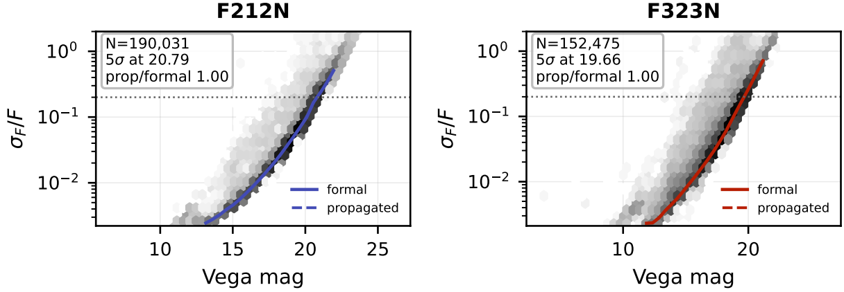
Figure 4: Photometric precision of quintuplet. Greyscale is source density; the solid line is the running median of the fitter’s formal uncertainty \sigma_F/F and the dashed line the same quantity propagated from the per-exposure scatter. The dotted horizontal line is \sigma_F/F = 0.2 , and where the median crosses it is quoted as the 5\sigma depth. A propagated-to-formal ratio above unity means the exposures disagree by more than the fit covariance predicts.
