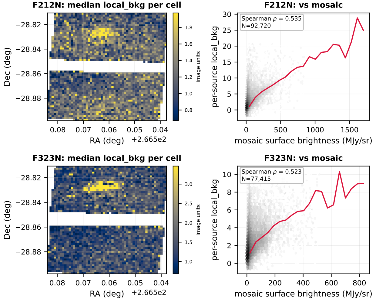
Figure 8: Spatial background structure in quintuplet. Left column: the median per-source background in 56 \times 56 sky cells – a map of the diffuse emission built entirely from the star catalogue. Right column: the same per-source value against the surface brightness of the drizzled mosaic sampled at that source’s position, with the running median in red and the Spearman rank correlation quoted. A high rank correlation is the evidence that the per-source background is measuring the astrophysical extended emission rather than a fitting artefact.
