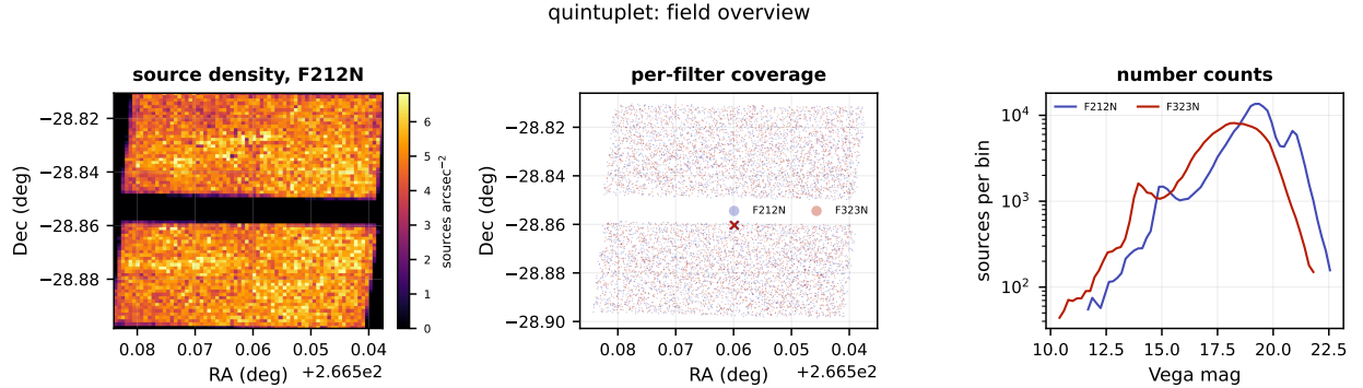
Figure 1: Overview of quintuplet. Left: source surface density in 72 \times 72 sky cells for F212N, the filter with the most detections. Centre: the sky coverage of each filter, sub-sampled. Right: number counts per filter; the peak of each curve is the turnover magnitude, the practical completeness limit beyond which the counts are set by detectability rather than by the stellar population.
