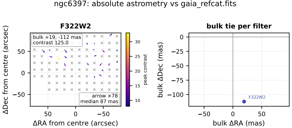
Figure 3: Absolute astrometry of ngc6397 against its registered reference catalogue. Each per-filter panel maps the offset-histogram tie on a 12 \times 12 tile grid (arrows, exaggerated; colour is the per-tile peak contrast), with the whole-field bulk tie quoted in the corner. Grey crosses mark tiles whose tie was only found by widening the search window and whose offset is therefore not trustworthy. The final panel collects the bulk ties. Offsets are measured by offset-histogram stacking, which is immune to the nearest-neighbour pairing collapse that a median against a dense reference suffers; the per-tile map is shown because a bulk offset near zero does not by itself mean the field is registered.
