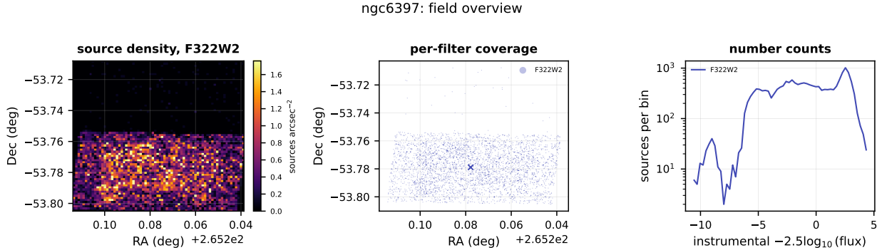
Figure 1: Overview of ngc6397. Left: source surface density in 72 \times 72 sky cells for F322W2, the filter with the most detections. Centre: the sky coverage of each filter, sub-sampled. Right: number counts per filter; the peak of each curve is the turnover magnitude, the practical completeness limit beyond which the counts are set by detectability rather than by the stellar population.
