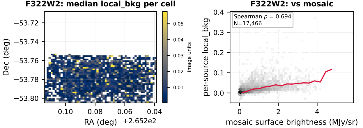
Figure 7: Spatial background structure in ngc6397. Left column: the median per-source background in 56 \times 56 sky cells – a map of the diffuse emission built entirely from the star catalogue. Right column: the same per-source value against the surface brightness of the drizzled mosaic sampled at that source’s position, with the running median in red and the Spearman rank correlation quoted. A high rank correlation is the evidence that the per-source background is measuring the astrophysical extended emission rather than a fitting artefact.
