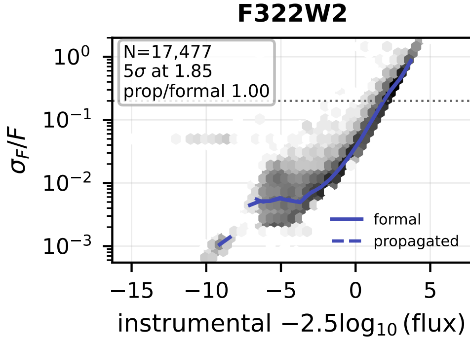
Figure 4: Photometric precision of ngc6397. Greyscale is source density; the solid line is the running median of the fitter’s formal uncertainty \sigma_F/F and the dashed line the same quantity propagated from the per-exposure scatter. The dotted horizontal line is \sigma_F/F = 0.2 , and where the median crosses it is quoted as the 5\sigma depth. A propagated-to-formal ratio above unity means the exposures disagree by more than the fit covariance predicts.
