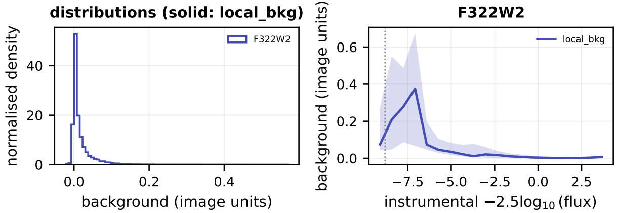
Figure 6: Background estimators for ngc6397. First panel: the distribution of the annulus background handed to the fitter (solid) and, where available, the residual-footprint background (dashed). Remaining panels: the running median of each against brightness, with the 16–84th percentile band for the annulus estimator; the vertical dotted line marks the brightest 1 per cent, where a star’s own wings begin to enter its own background aperture. The residual-footprint column is present for 0 of 1 filters; it was added in 2026-07, so catalogues produced before then carry only the annulus estimator.
