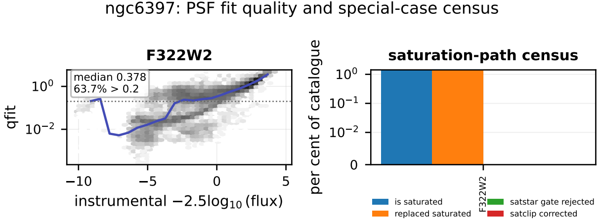
Figure 5: PSF-fit quality for ngc6397. Per filter, the normalised fit residual qfit against brightness (greyscale: source density; line: running median; dotted: the qfit = 0.2 vetting threshold). The final panel is the fraction of each filter’s catalogue touched by the saturation-handling paths: flagged saturated, core-replaced, rejected by the saturated-star gate, and clip-corrected.
