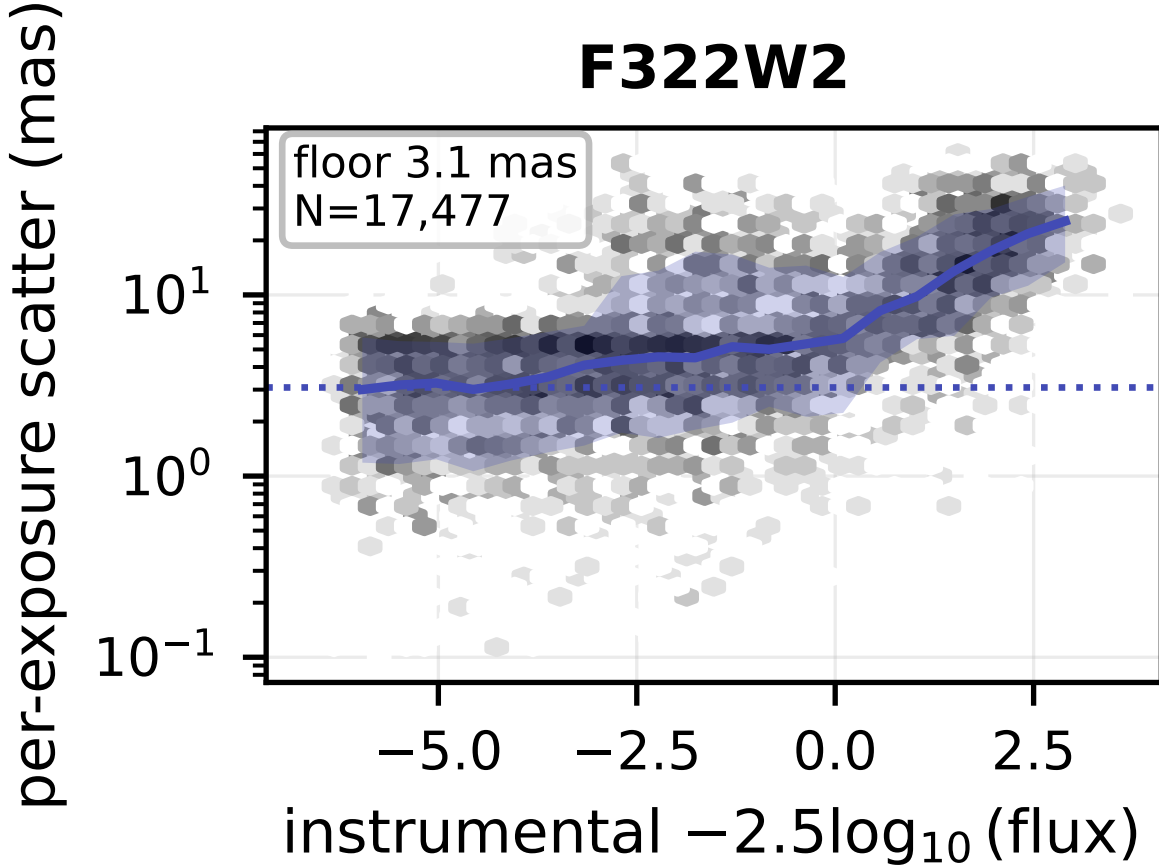
Figure 2: Internal astrometry of ngc6397. Per filter: the scatter of the individual-exposure centroids about the merged position, against brightness; greyscale is source density, the coloured line and band are the running median and 16–84th percentile, and the dotted line marks the bright-decile floor quoted in the panel.
