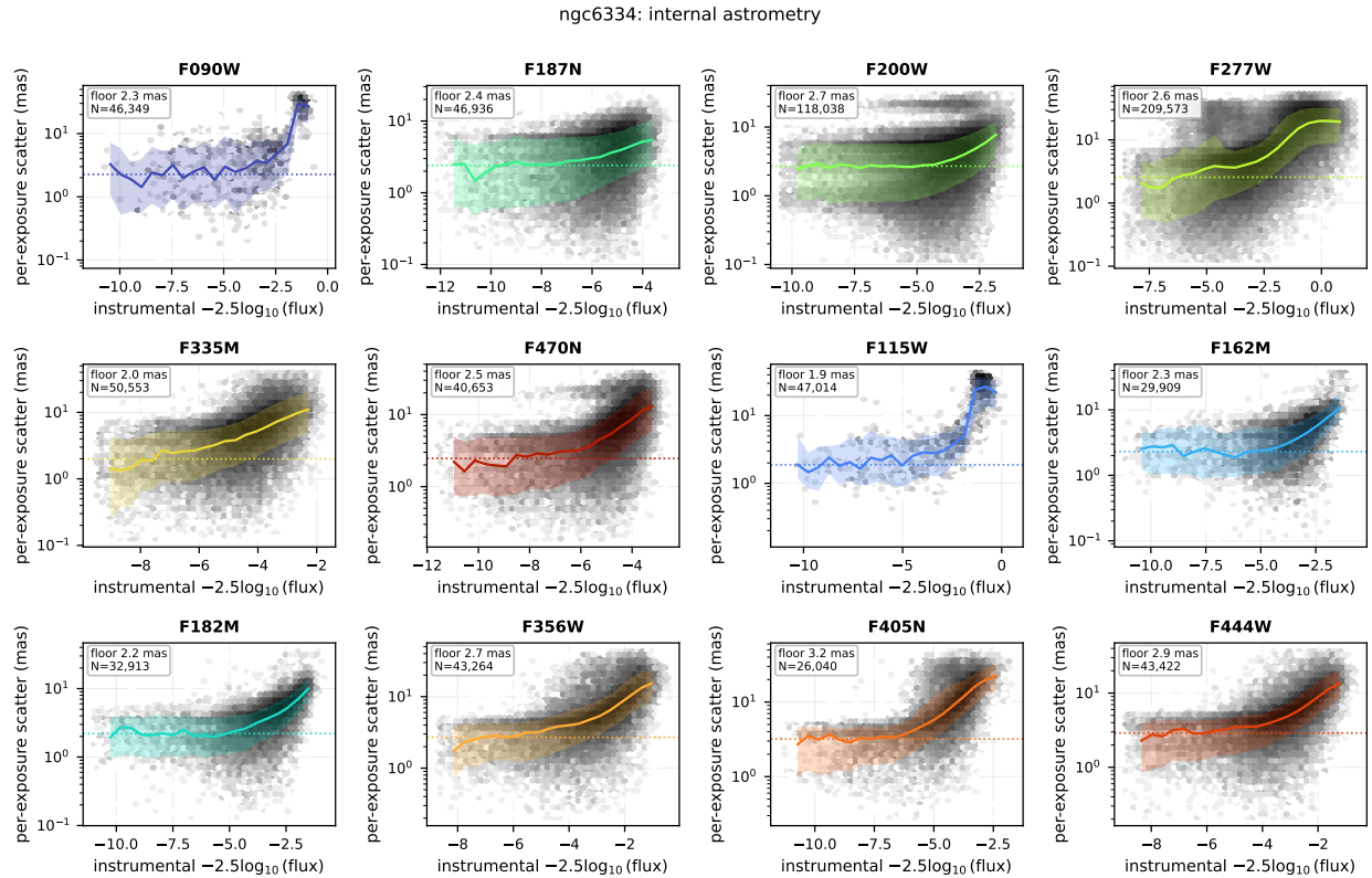
Figure 2: Internal astrometry of ngc6334. Per filter: the scatter of the individual-exposure centroids about the merged position, against brightness; greyscale is source density, the coloured line and band are the running median and 16–84th percentile, and the dotted line marks the bright-decile floor quoted in the panel.
