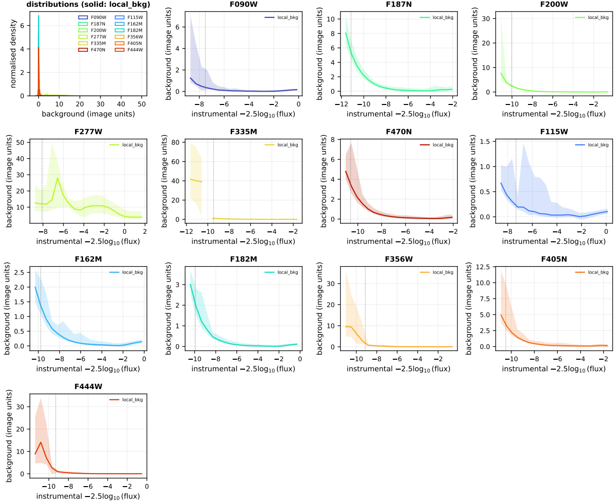
Figure 6: Background estimators for ngc6334. First panel: the distribution of the annulus background handed to the fitter (solid) and, where available, the residual-footprint background (dashed). Remaining panels: the running median of each against brightness, with the 16–84th percentile band for the annulus estimator; the vertical dotted line marks the brightest 1 per cent, where a star’s own wings begin to enter its own background aperture. The residual-footprint column is present for 0 of 12 filters; it was added in 2026-07, so catalogues produced before then carry only the annulus estimator.
