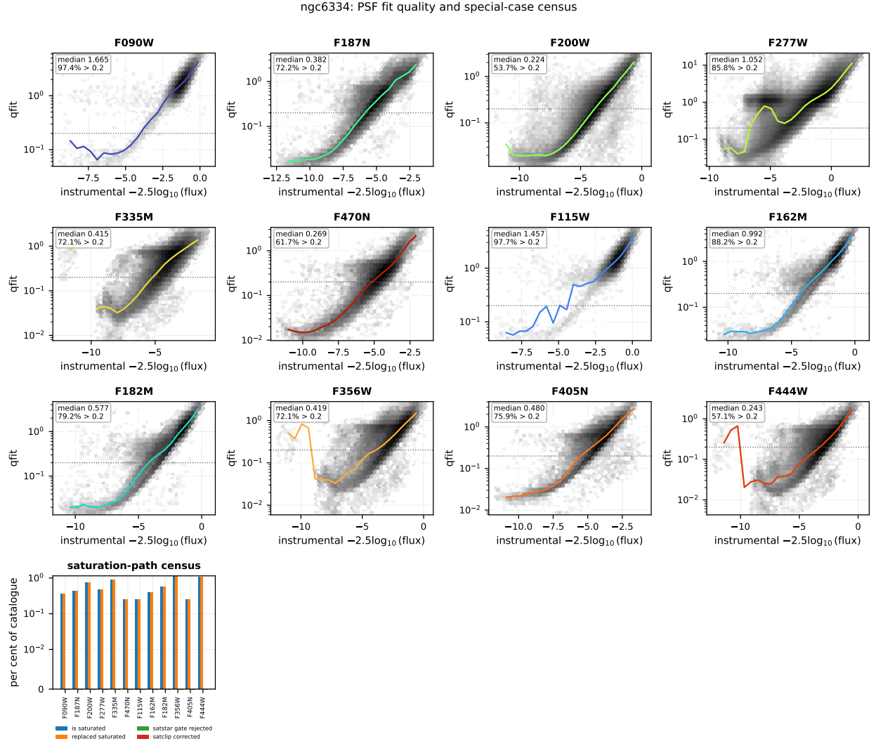
Figure 5: PSF-fit quality for ngc6334. Per filter, the normalised fit residual q_{\text{fit}} against brightness (greyscale: source density; line: running median; dotted: the q_{\text{fit}} = 0.2 vetting threshold). The final panel is the fraction of each filter's catalogue touched by the saturation-handling paths: flagged saturated, core-replaced, rejected by the saturated-star gate, and clip-corrected.
