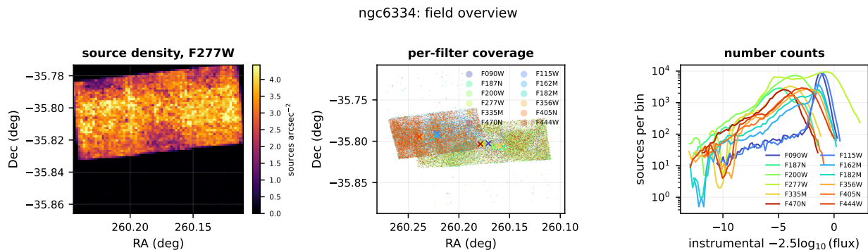
Figure 1: Overview of ngc6334. Left: source surface density in 72 \times 72 sky cells for F277W, the filter with the most detections. Centre: the sky coverage of each filter, sub-sampled. Right: number counts per filter; the peak of each curve is the turnover magnitude, the practical completeness limit beyond which the counts are set by detectability rather than by the stellar population.
