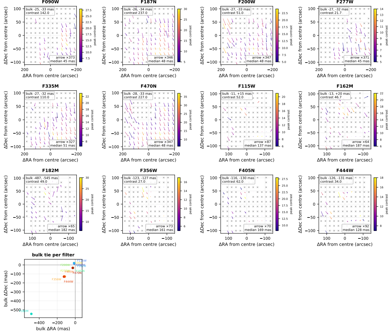
Figure 3: Absolute astrometry of ngc6334 against its registered reference catalogue. Each per-filter panel maps the offset-histogram tie on a 12 \times 12 tile grid (arrows, exaggerated; colour is the per-tile peak contrast), with the whole-field bulk tie quoted in the corner. Grey crosses mark tiles whose tie was only found by widening the search window and whose offset is therefore not trustworthy. The final panel collects the bulk ties. Offsets are measured by offset-histogram stacking, which is immune to the nearest-neighbour pairing collapse that a median against a dense reference suffers; the per-tile map is shown because a bulk offset near zero does not by itself mean the field is registered.
