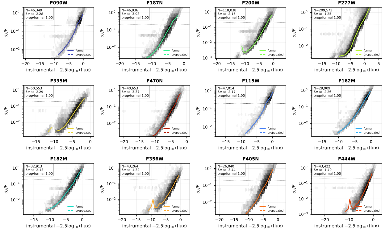
Figure 4: Photometric precision of ngc6334. Greyscale is source density; the solid line is the running median of the fitter’s formal uncertainty \sigma_F/F and the dashed line the same quantity propagated from the per-exposure scatter. The dotted horizontal line is \sigma_F/F = 0.2 , and where the median crosses it is quoted as the 5\sigma depth. A propagated-to-formal ratio above unity means the exposures disagree by more than the fit covariance predicts.
