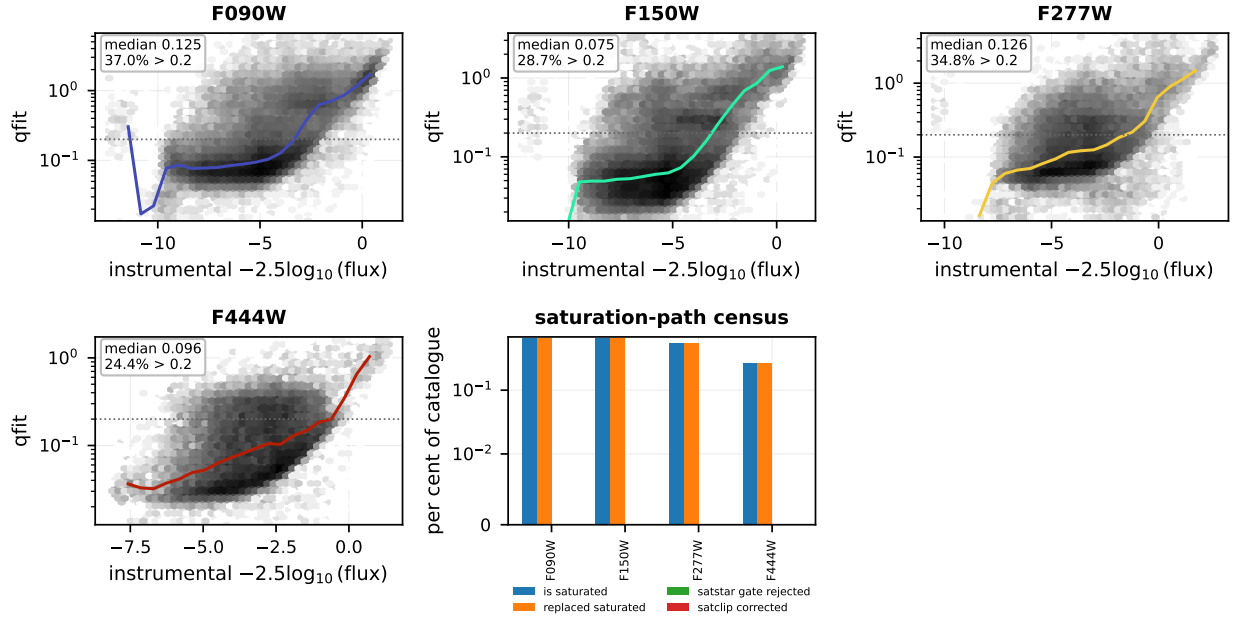
Figure 5: PSF-fit quality for m92. Per filter, the normalised fit residual q_{\text{fit}} against brightness (greyscale: source density; line: running median; dotted: the q_{\text{fit}} = 0.2 vetting threshold). The final panel is the fraction of each filter’s catalogue touched by the saturation-handling paths: flagged saturated, core-replaced, rejected by the saturated-star gate, and clip-corrected.
