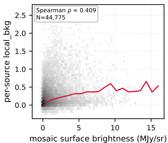
F444W: vs mosaic
