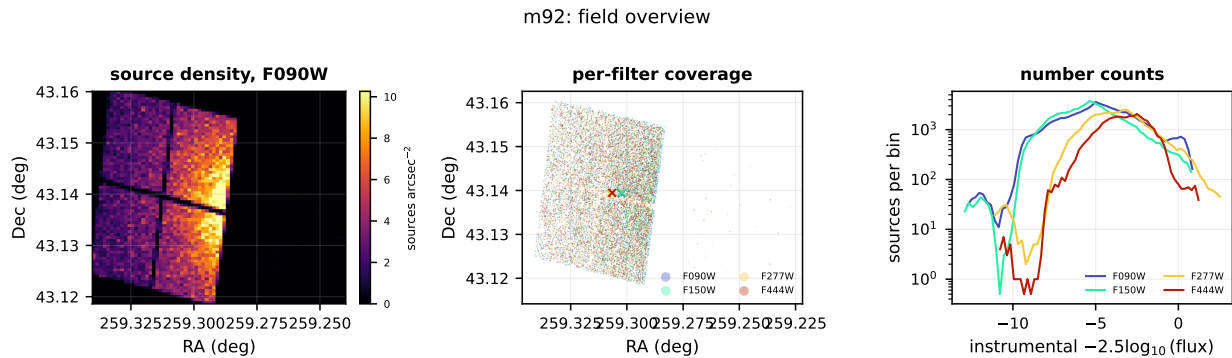
Figure 1: Overview of m92. Left: source surface density in 72 \times 72 sky cells for F090W, the filter with the most detections. Centre: the sky coverage of each filter, sub-sampled. Right: number counts per filter; the peak of each curve is the turnover magnitude, the practical completeness limit beyond which the counts are set by detectability rather than by the stellar population.
