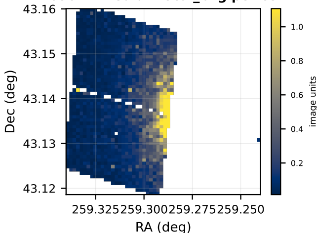
F150W: median local_bkg per cell
