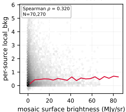
F150W: vs mosaic
