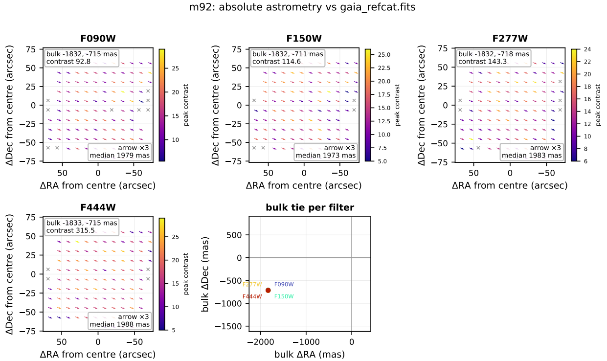
Figure 3: Absolute astrometry of m92 against its registered reference catalogue. Each per-filter panel maps the offset-histogram tie on a 12 \times 12 tile grid (arrows, exaggerated; colour is the per-tile peak contrast), with the whole-field bulk tie quoted in the corner. Grey crosses mark tiles whose tie was only found by widening the search window and whose offset is therefore not trustworthy. The final panel collects the bulk ties. Offsets are measured by offset-histogram stacking, which is immune to the nearest-neighbour pairing collapse that a median against a dense reference suffers; the per-tile map is shown because a bulk offset near zero does not by itself mean the field is registered.
