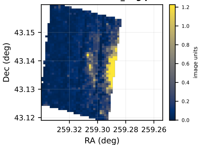
F444W: median local_bkg per cell
