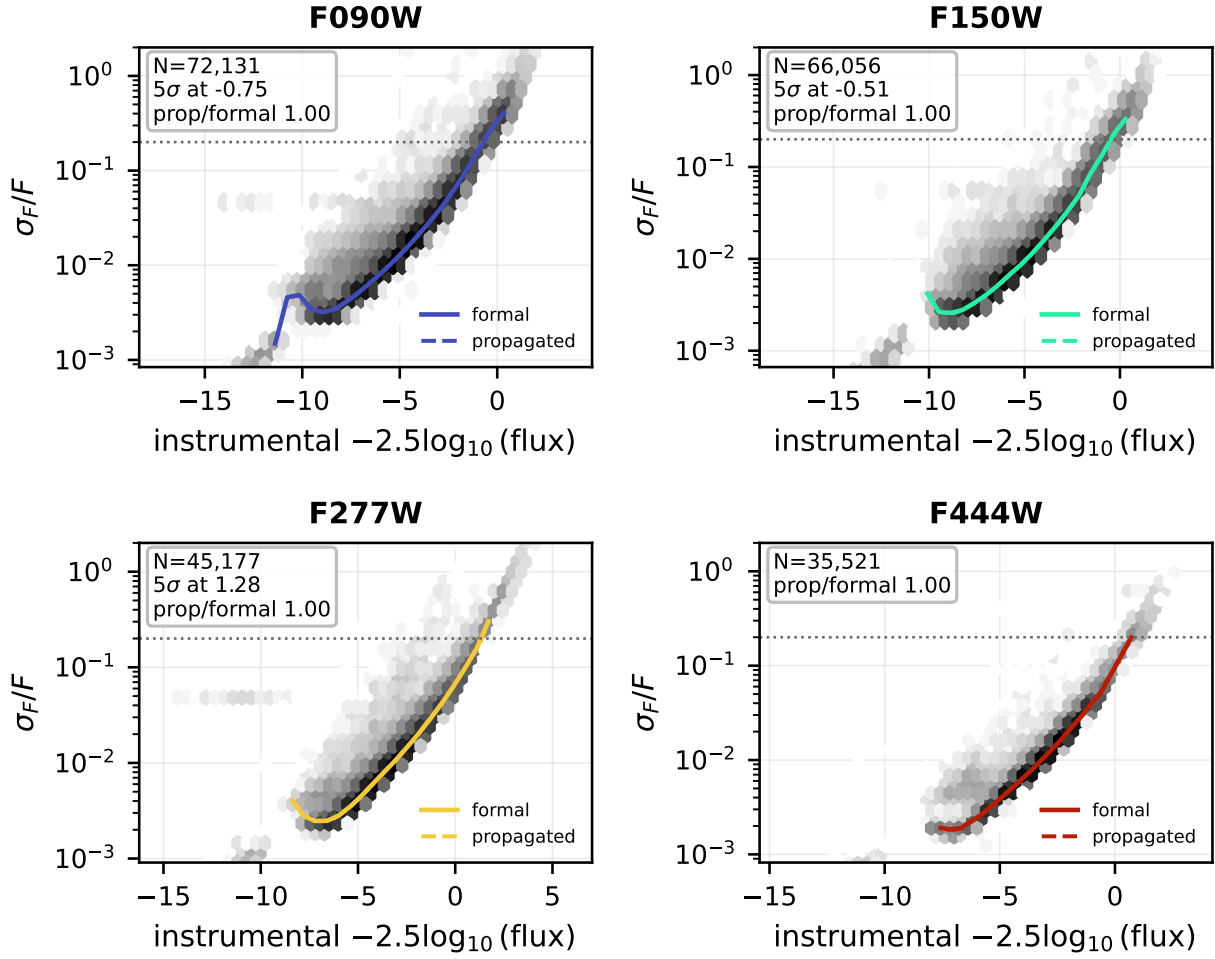
Figure 4: Photometric precision of m92. Greyscale is source density; the solid line is the running median of the fitter’s formal uncertainty \sigma_F/F and the dashed line the same quantity propagated from the per-exposure scatter. The dotted horizontal line is \sigma_F/F = 0.2 , and where the median crosses it is quoted as the 5\sigma depth. A propagated-to-formal ratio above unity means the exposures disagree by more than the fit covariance predicts.
