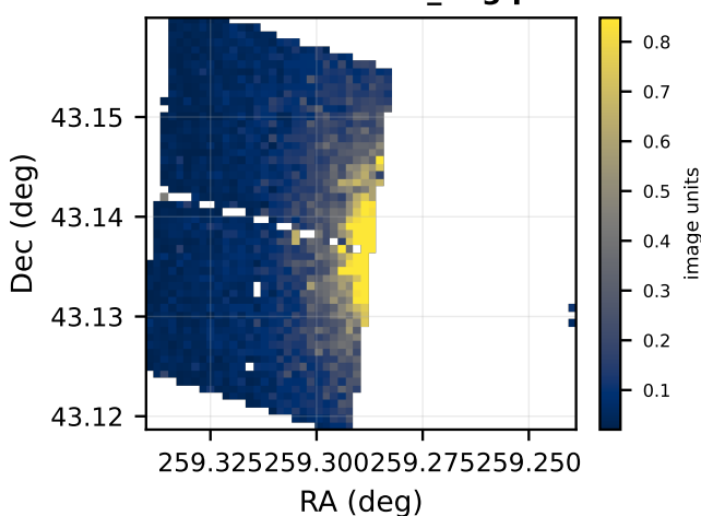
F277W: median local_bkg per cell
