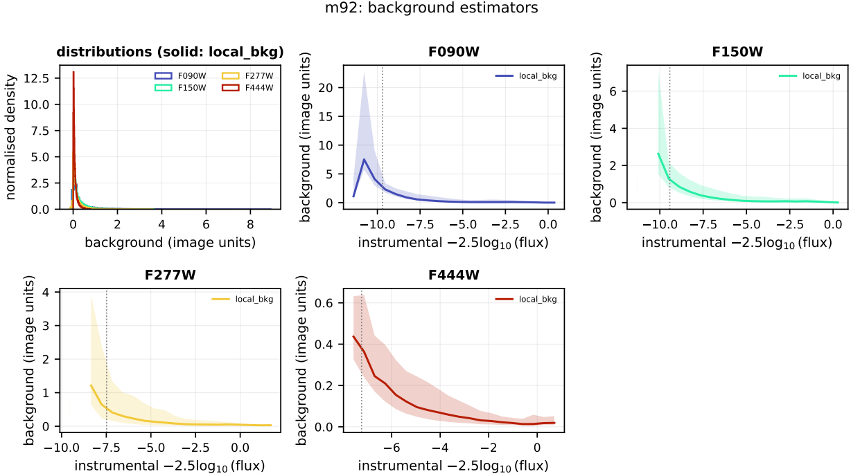
Figure 6: Background estimators for m92. First panel: the distribution of the annulus background handed to the fitter (solid) and, where available, the residual-footprint background (dashed). Remaining panels: the running median of each against brightness, with the 16–84th percentile band for the annulus estimator; the vertical dotted line marks the brightest 1 per cent, where a star’s own wings begin to enter its own background aperture. The residual-footprint column is present for 0 of 4 filters; it was added in 2026-07, so catalogues produced before then carry only the annulus estimator.
