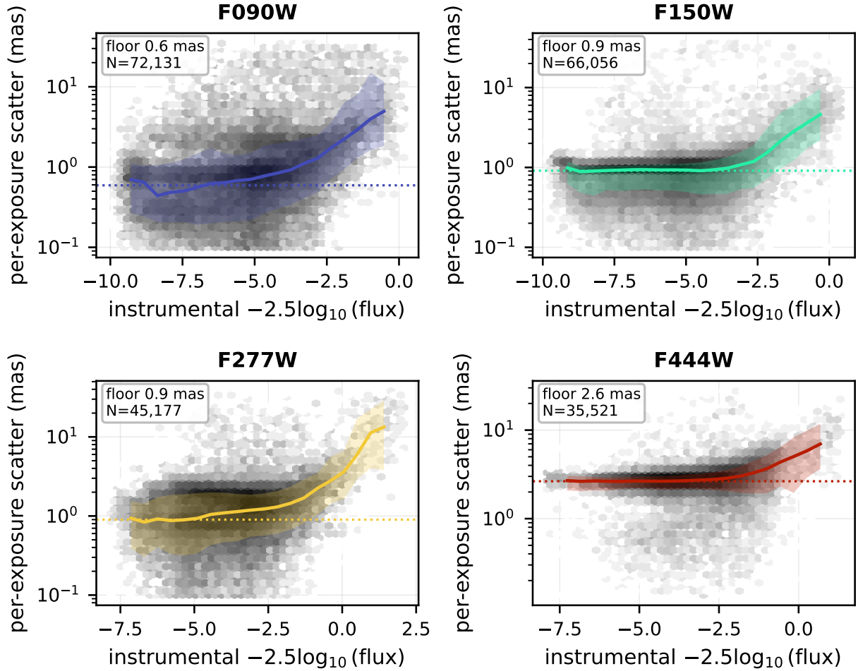
Figure 2: Internal astrometry of m92. Per filter: the scatter of the individual-exposure centroids about the merged position, against brightness; greyscale is source density, the coloured line and band are the running median and 16–84th percentile, and the dotted line marks the bright-decile floor quoted in the panel.
