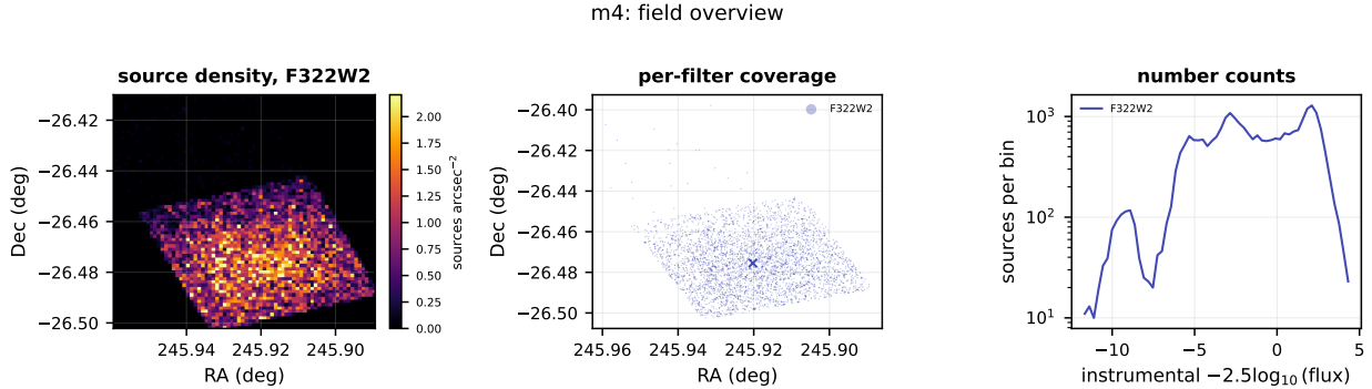
Figure 1: Overview of m4. Left: source surface density in 72 \times 72 sky cells for F322W2, the filter with the most detections. Centre: the sky coverage of each filter, sub-sampled. Right: number counts per filter; the peak of each curve is the turnover magnitude, the practical completeness limit beyond which the counts are set by detectability rather than by the stellar population.
