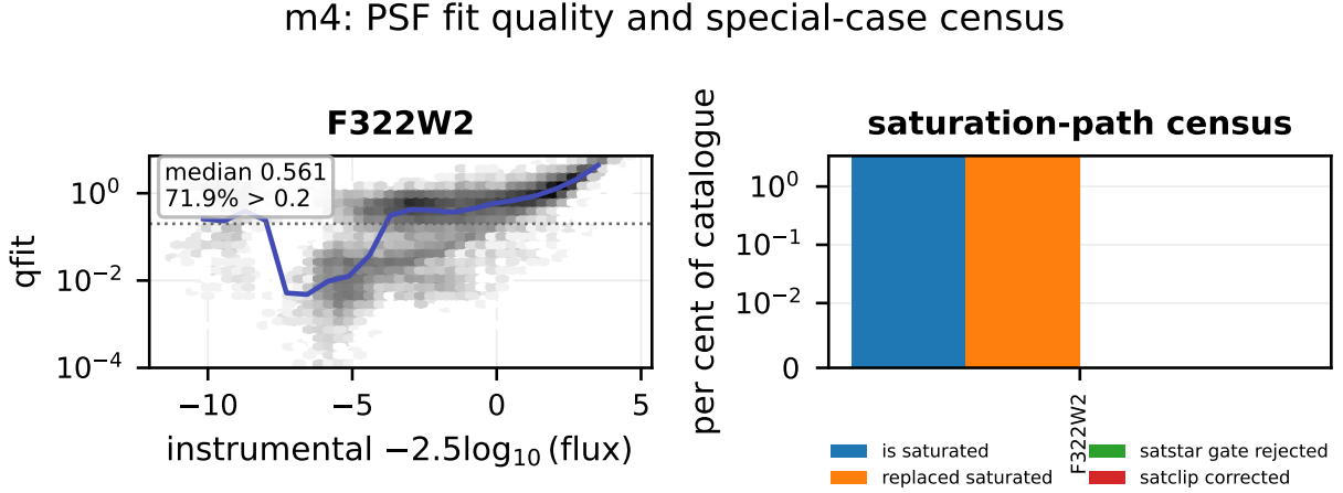
Figure 5: PSF-fit quality for m4. Per filter, the normalised fit residual qfit against brightness (greyscale: source density; line: running median; dotted: the qfit = 0.2 vetting threshold). The final panel is the fraction of each filter’s catalogue touched by the saturation-handling paths: flagged saturated, core-replaced, rejected by the saturated-star gate, and clip-corrected.
