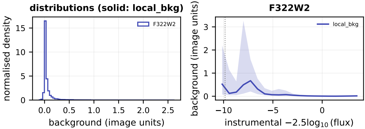
Figure 6: Background estimators for m4. First panel: the distribution of the annulus background handed to the fitter (solid) and, where available, the residual-footprint background (dashed). Remaining panels: the running median of each against brightness, with the 16–84th percentile band for the annulus estimator; the vertical dotted line marks the brightest 1 per cent, where a star’s own wings begin to enter its own background aperture. The residual-footprint column is present for 0 of 1 filters; it was added in 2026-07, so catalogues produced before then carry only the annulus estimator.
