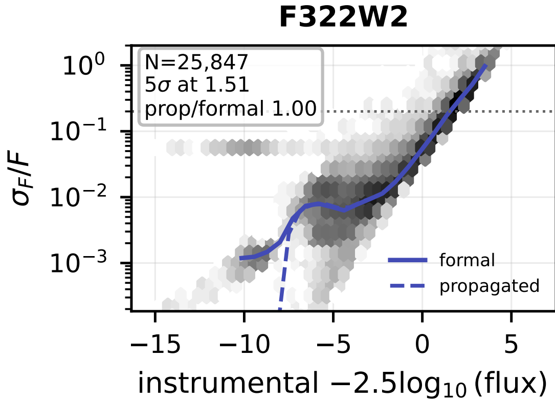
Figure 4: Photometric precision of m4. Greyscale is source density; the solid line is the running median of the fitter’s formal uncertainty \sigma_F/F and the dashed line the same quantity propagated from the per-exposure scatter. The dotted horizontal line is \sigma_F/F = 0.2 , and where the median crosses it is quoted as the 5\sigma depth. A propagated-to-formal ratio above unity means the exposures disagree by more than the fit covariance predicts.
