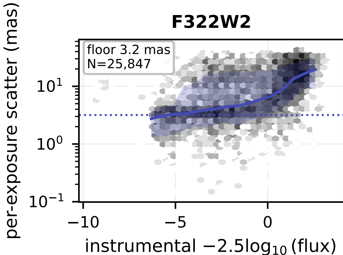
Figure 2: Internal astrometry of m4. Per filter: the scatter of the individual-exposure centroids about the merged position, against brightness; greyscale is source density, the coloured line and band are the running median and 16–84th percentile, and the dotted line marks the bright-decile floor quoted in the panel.
