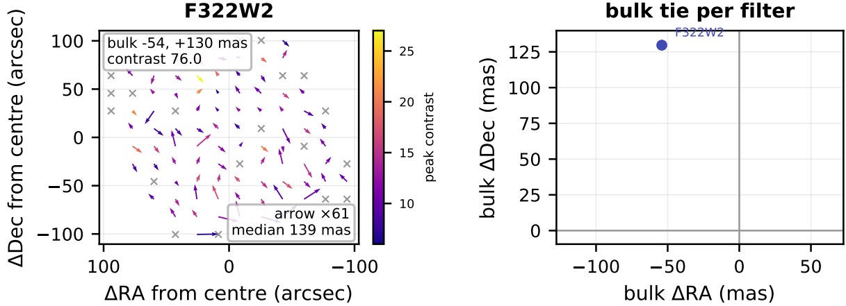
Figure 3: Absolute astrometry of m4 against its registered reference catalogue. Each per-filter panel maps the offset-histogram tie on a 12 \times 12 tile grid (arrows, exaggerated; colour is the per-tile peak contrast), with the whole-field bulk tie quoted in the corner. Grey crosses mark tiles whose tie was only found by widening the search window and whose offset is therefore not trustworthy. The final panel collects the bulk ties. Offsets are measured by offset-histogram stacking, which is immune to the nearest-neighbour pairing collapse that a median against a dense reference suffers; the per-tile map is shown because a bulk offset near zero does not by itself mean the field is registered.
