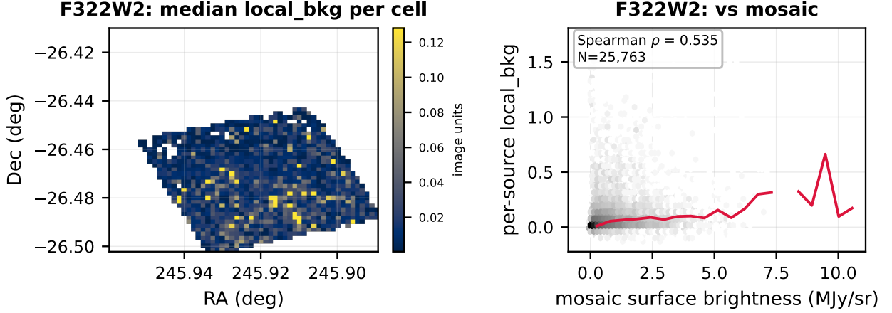
Figure 7: Spatial background structure in m4. Left column: the median per-source background in 56 \times 56 sky cells – a map of the diffuse emission built entirely from the star catalogue. Right column: the same per-source value against the surface brightness of the drizzled mosaic sampled at that source’s position, with the running median in red and the Spearman rank correlation quoted. A high rank correlation is the evidence that the per-source background is measuring the astrophysical extended emission rather than a fitting artefact.
