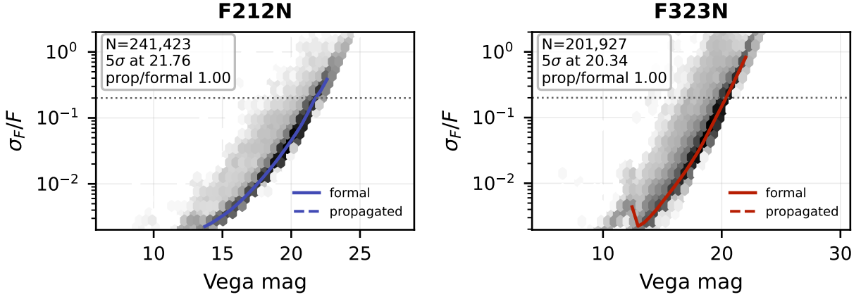
Figure 4: Photometric precision of arches. Greyscale is source density; the solid line is the running median of the fitter’s formal uncertainty \sigma_F/F and the dashed line the same quantity propagated from the per-exposure scatter. The dotted horizontal line is \sigma_F/F = 0.2 , and where the median crosses it is quoted as the 5\sigma depth. A propagated-to-formal ratio above unity means the exposures disagree by more than the fit covariance predicts.
