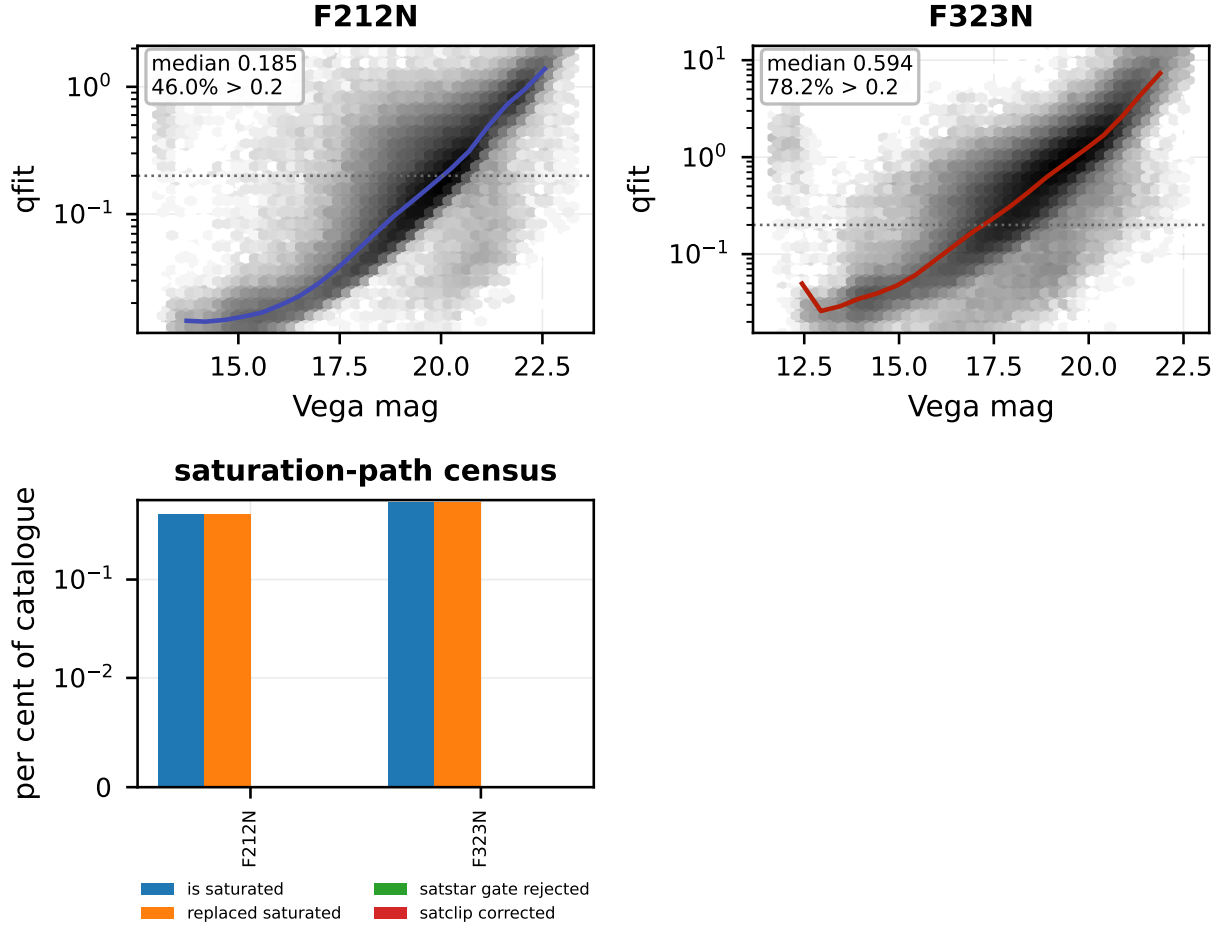
Figure 5: PSF-fit quality for arches. Per filter, the normalised fit residual qfit against brightness (greyscale: source density; line: running median; dotted: the qfit = 0.2 vetting threshold). The final panel is the fraction of each filter’s catalogue touched by the saturation-handling paths: flagged saturated, core-replaced, rejected by the saturated-star gate, and clip-corrected.
