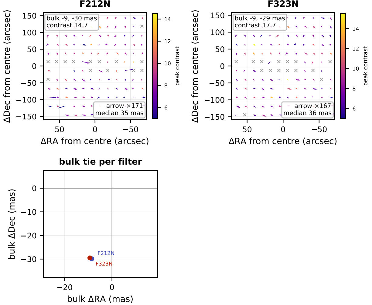
Figure 3: Absolute astrometry of arches against its registered reference catalogue. Each per-filter panel maps the offset-histogram tie on a 12 \times 12 tile grid (arrows, exaggerated; colour is the per-tile peak contrast), with the whole-field bulk tie quoted in the corner. Grey crosses mark tiles whose tie was only found by widening the search window and whose offset is therefore not trustworthy. The final panel collects the bulk ties. Offsets are measured by offset-histogram stacking, which is immune to the nearest-neighbour pairing collapse that a median against a dense reference suffers; the per-tile map is shown because a bulk offset near zero does not by itself mean the field is registered.
