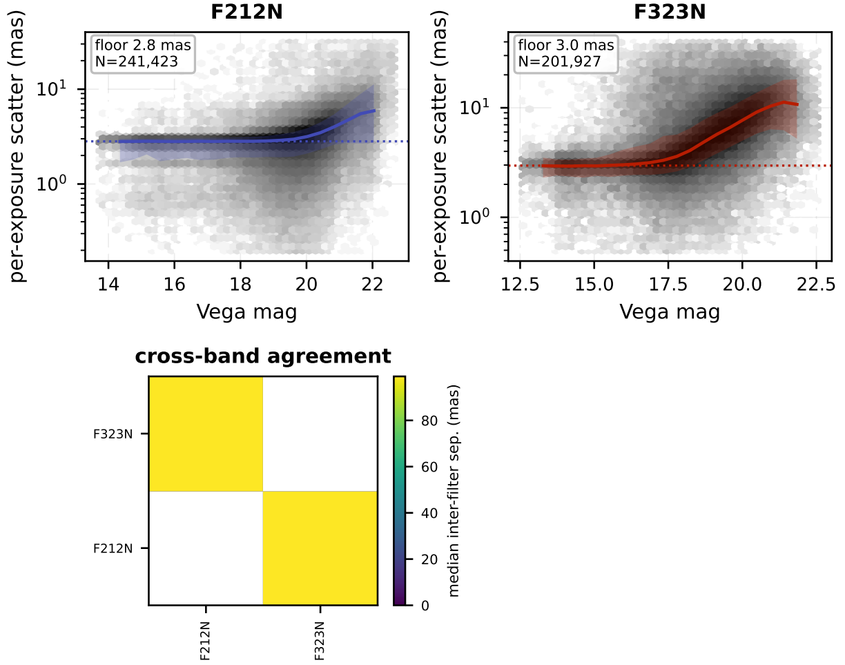
Figure 2: Internal astrometry of arches. Per filter: the scatter of the individual-exposure centroids about the merged position, against brightness; greyscale is source density, the coloured line and band are the running median and 16–84th percentile, and the dotted line marks the bright-decile floor quoted in the panel. The final panel is the median separation between the same stars measured independently in each pair of filters; only sources independently detected in both bands are counted, since a forced or seeded position imported from another band would measure the merge radius rather than the astrometry.
