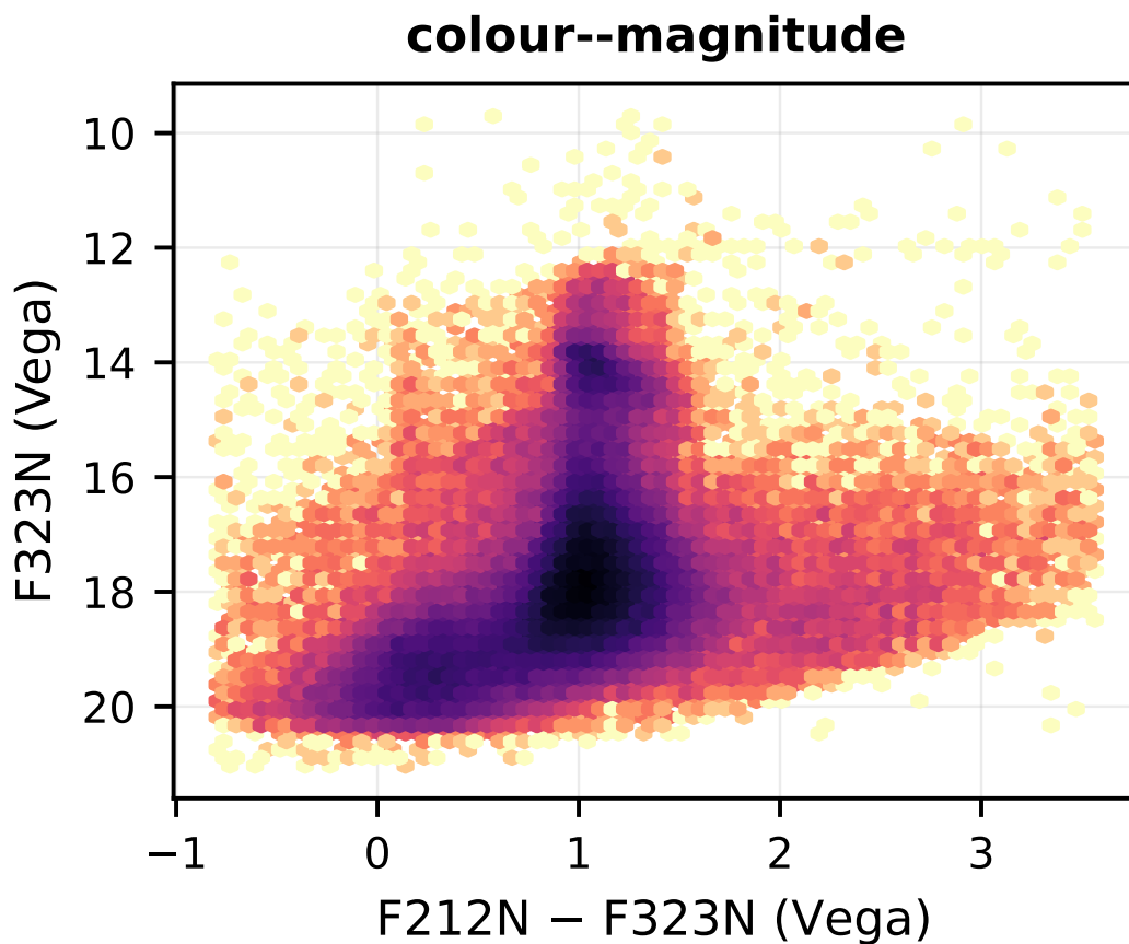
Figure 6: Colour diagrams for arches, from the stage-m7 cross-band merge, in Vega magnitudes. These are differential between filters and so respond to systematics that per-filter statistics cannot see: a zero-point error shifts a sequence bodily, a saturation-correction discontinuity breaks it at a specific magnitude, and a filter-dependent background error tilts it.
