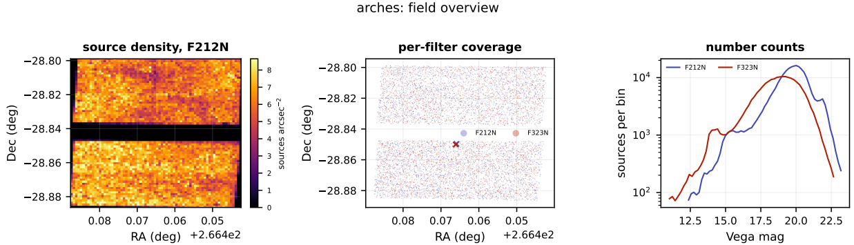
Figure 1: Overview of arches. Left: source surface density in 72 \times 72 sky cells for F212N, the filter with the most detections. Centre: the sky coverage of each filter, sub-sampled. Right: number counts per filter; the peak of each curve is the turnover magnitude, the practical completeness limit beyond which the counts are set by detectability rather than by the stellar population.
