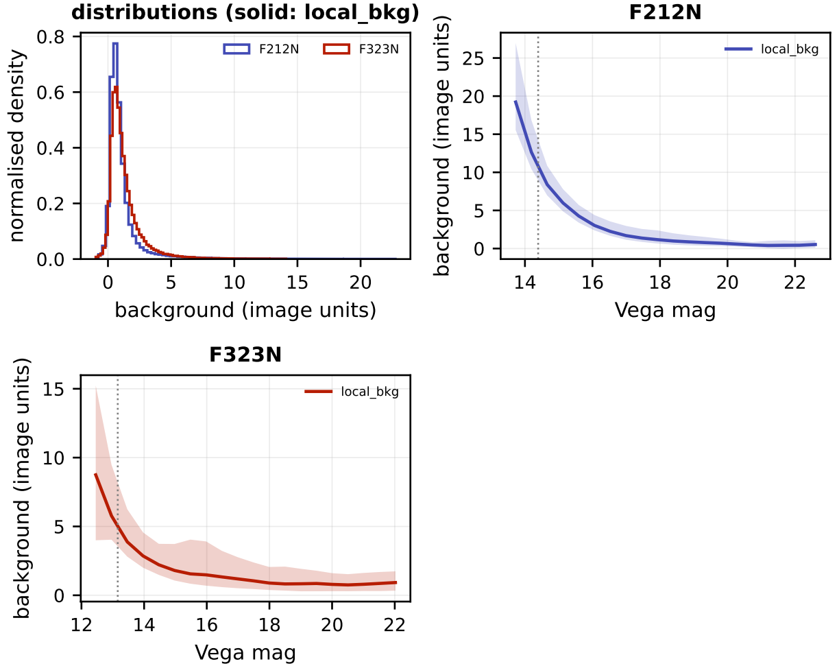
Figure 7: Background estimators for arches. First panel: the distribution of the annulus background handed to the fitter (solid) and, where available, the residual-footprint background (dashed). Remaining panels: the running median of each against brightness, with the 16–84th percentile band for the annulus estimator; the vertical dotted line marks the brightest 1 per cent, where a star’s own wings begin to enter its own background aperture. The residual-footprint column is present for 0 of 2 filters; it was added in 2026-07, so catalogues produced before then carry only the annulus estimator.
