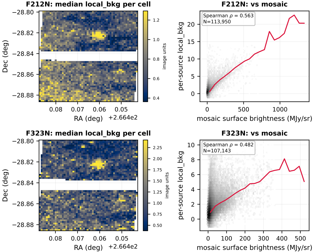
Figure 8: Spatial background structure in arches. Left column: the median per-source background in 56 \times 56 sky cells – a map of the diffuse emission built entirely from the star catalogue. Right column: the same per-source value against the surface brightness of the drizzled mosaic sampled at that source’s position, with the running median in red and the Spearman rank correlation quoted. A high rank correlation is the evidence that the per-source background is measuring the astrophysical extended emission rather than a fitting artefact.
